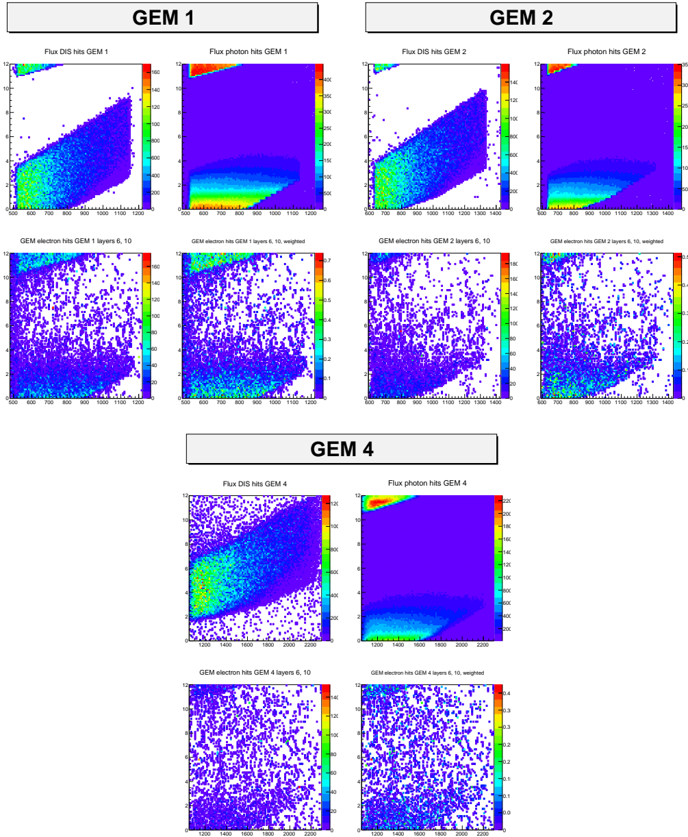
FIGURE 2. (Top plots) Hit positions of high x_{bj} DIS electrons (left) and from GEANT generator data (right) in virtual flux detectors in front of GEMs 1, 2 and 4. (Bottom plots) Positions in GEM gas layers of electrons and positrons from GEANT generator data, unweighted (left) and weighted by deposited energy in the gas (right).
