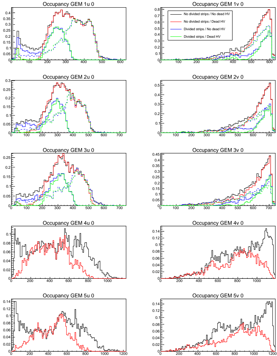
FIGURE 3. Occupancies versus strip number, for each of five GEMs (rows) and two strip orientations (columns). Red and green lines are with dead HV regions; blue and green lines are with divided strips. Solid (dashed) lines are for substrip 0 (1).
