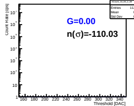
Pmt 3 Pixel 61
