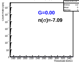
Pmt 2 Pixel 56
