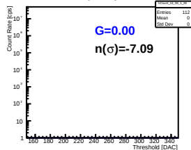
Pmt 2 Pixel 9
