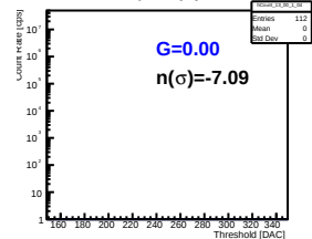
Pmt 2 Pixel 52
