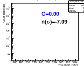
Pmt 2 Pixel 16
