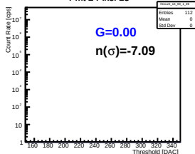
Pmt 2 Pixel 13
