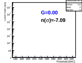
Pmt 2 Pixel 22
