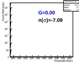
Pmt 2 Pixel 49
