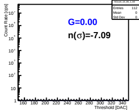
Pmt 2 Pixel 43
