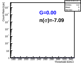
Pmt 2 Pixel 28
