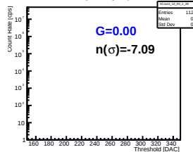
Pmt 2 Pixel 15
