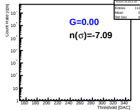
Pmt 2 Pixel 5
