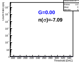
Pmt 2 Pixel 45
