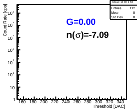
Pmt 3 Pixel 59
