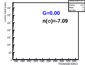
Pmt 2 Pixel 27
