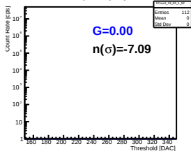
Pmt 2 Pixel 50
