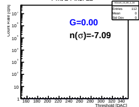
Pmt 2 Pixel 12
