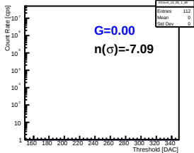
Pmt 2 Pixel 44
