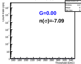
Pmt 2 Pixel 55
