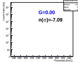
Pmt 2 Pixel 6
