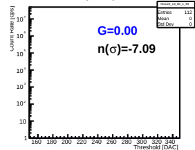
Pmt 2 Pixel 47
