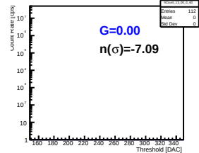
Pmt 2 Pixel 2
