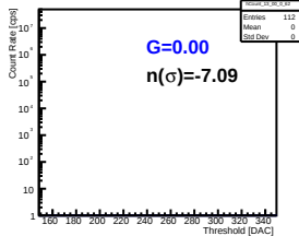
Pmt 2 Pixel 3
