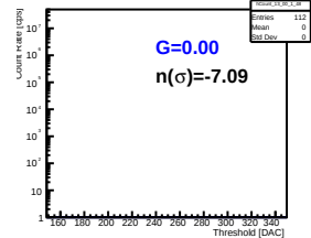
Pmt 2 Pixel 42
