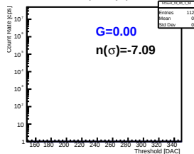
Pmt 2 Pixel 11
