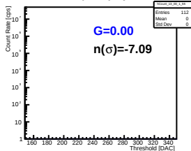
Pmt 2 Pixel 48
