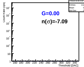
Pmt 3 Pixel 62
