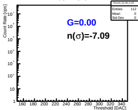
Pmt 3 Pixel 64
