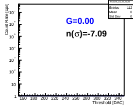
Pmt 2 Pixel 4
