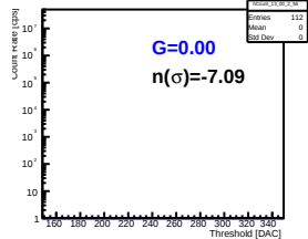
Pmt 3 Pixel 58
