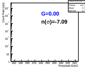
Pmt 2 Pixel 54
