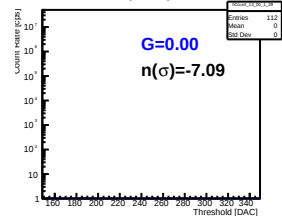
Pmt 2 Pixel 7
