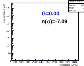
Pmt 2 Pixel 10
