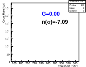
Pmt 2 Pixel 33
