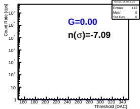
Pmt 2 Pixel 23
