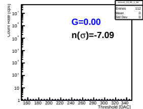
Pmt 2 Pixel 32
