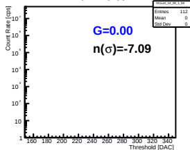
Pmt 2 Pixel 53
