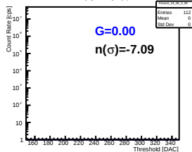
Pmt 3 Pixel 60
