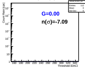
Pmt 2 Pixel 8
