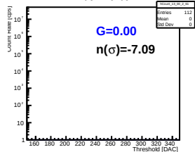
Pmt 3 Pixel 63
