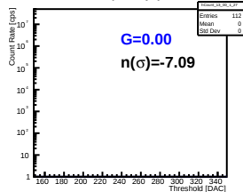
Pmt 2 Pixel 14
