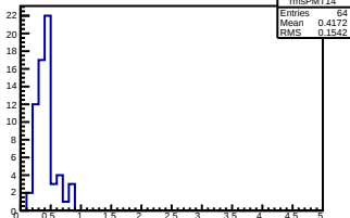
PMT 14, Pedestal RMS
