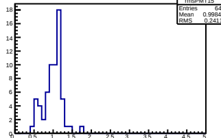
PMT 15, Pedestal RMS
