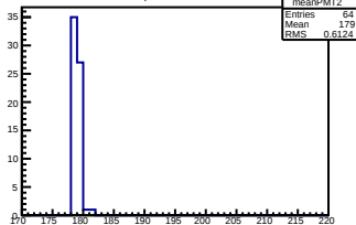
PMT 2, Pedestal Mean
