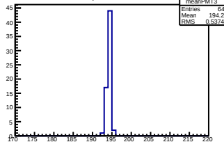
PMT 3, Pedestal Mean
