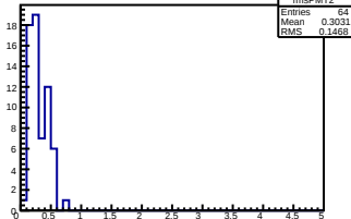
PMT 2, Pedestal RMS
