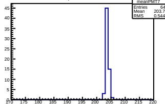
PMT 7, Pedestal Mean
