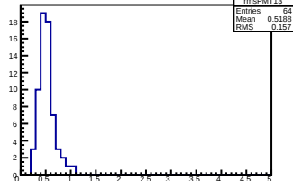
PMT 13, Pedestal RMS
