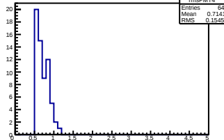
PMT 4, Pedestal RMS
