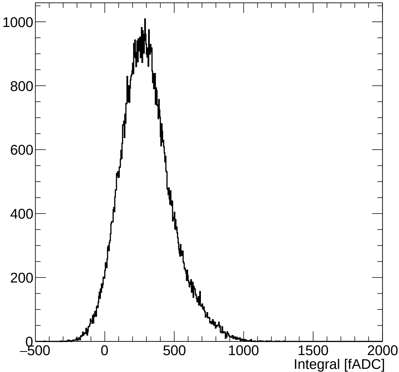
Integral Distribution (with pedestal subtraction)
