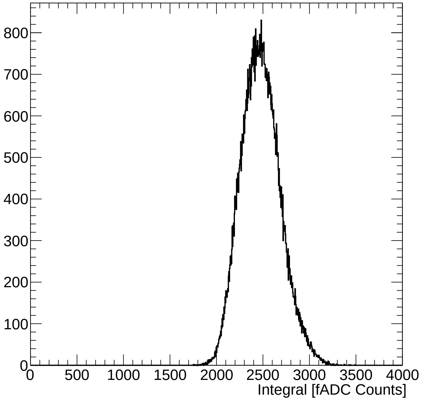
Integral Distribution (no pedestal subtraction)
