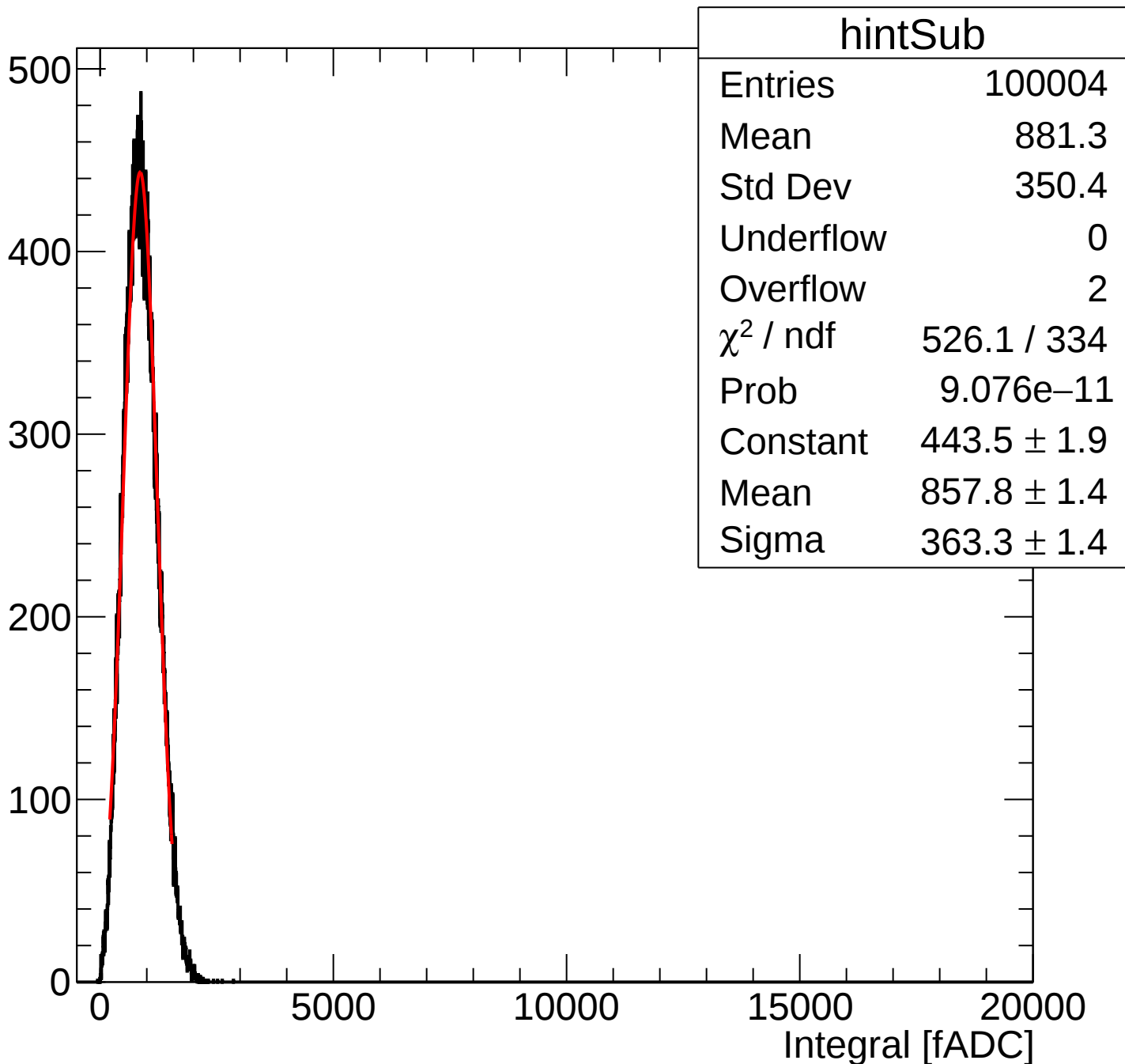
Integral Distribution (with pedestal subtraction)
