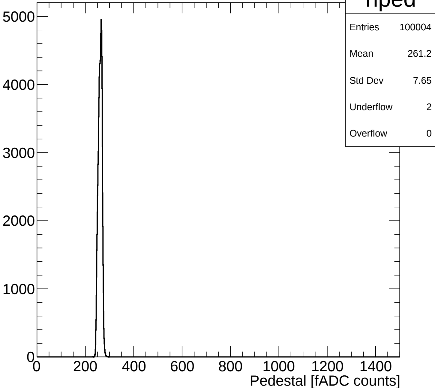
Pedestal Distribution (average fADC count between 52 - 88 ns)
