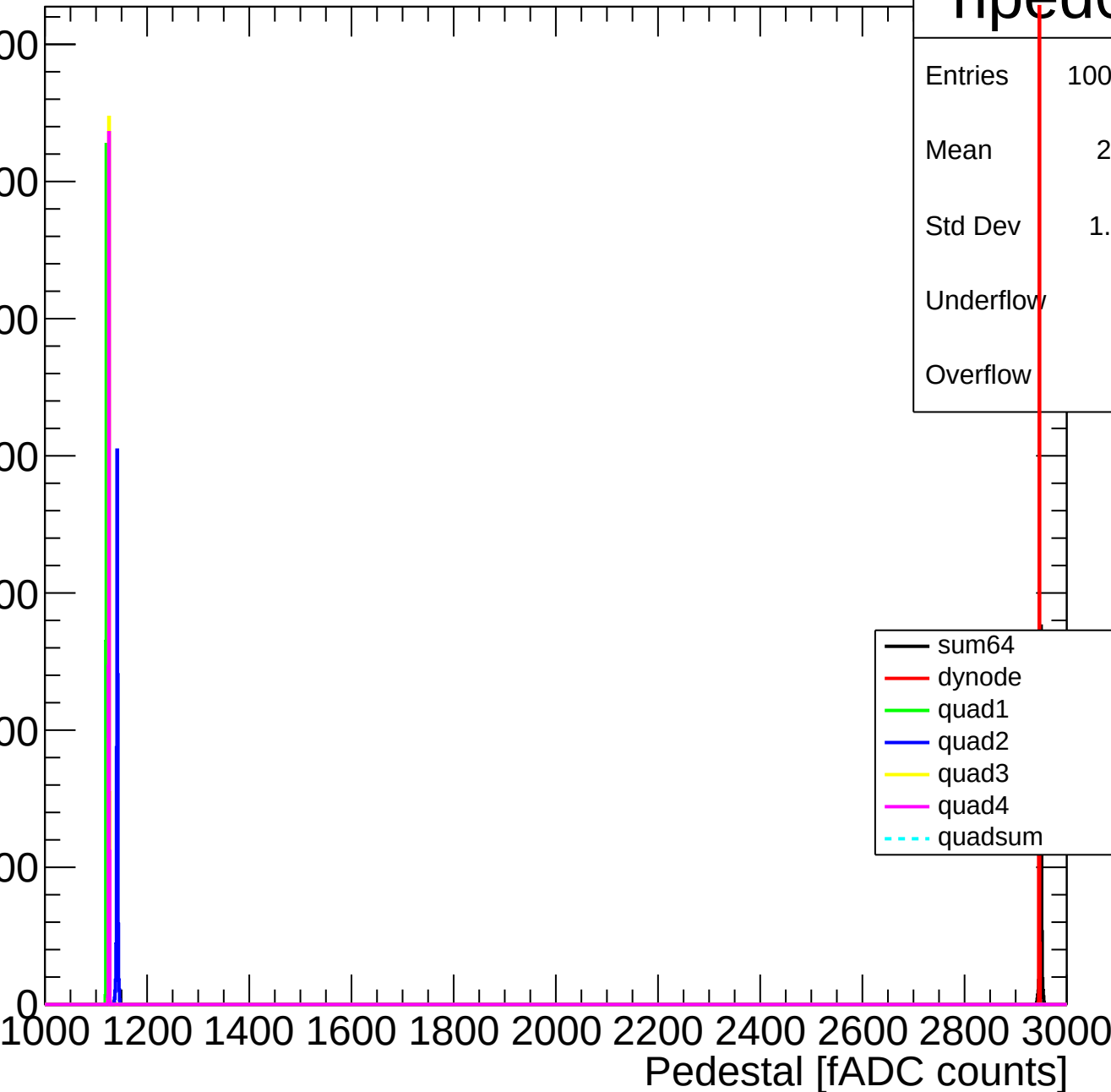
Pedestal Distribution (average fADC count between 8 - 80 ns)
