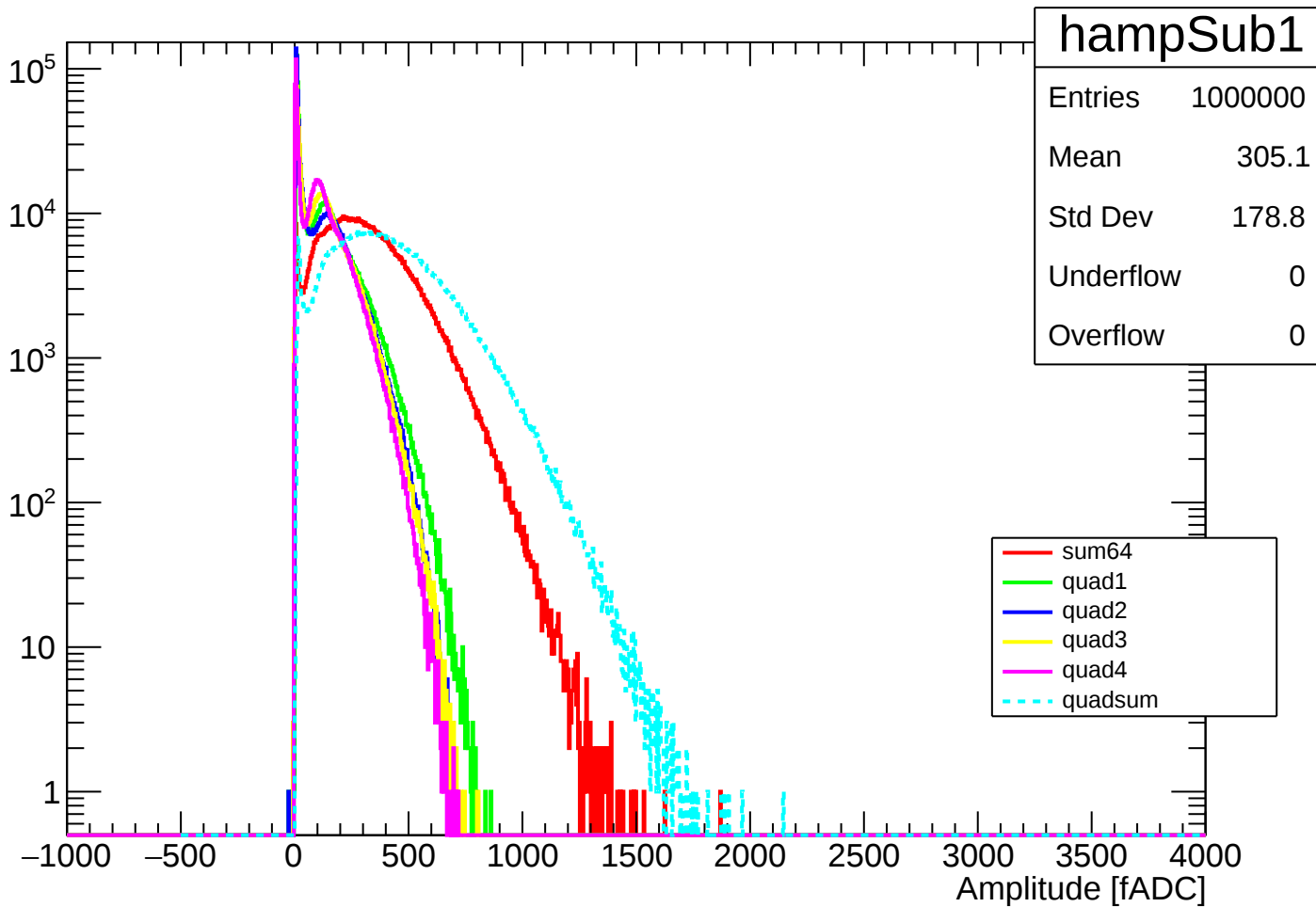
Amplitude Distribution (with pedestal subtraction)
