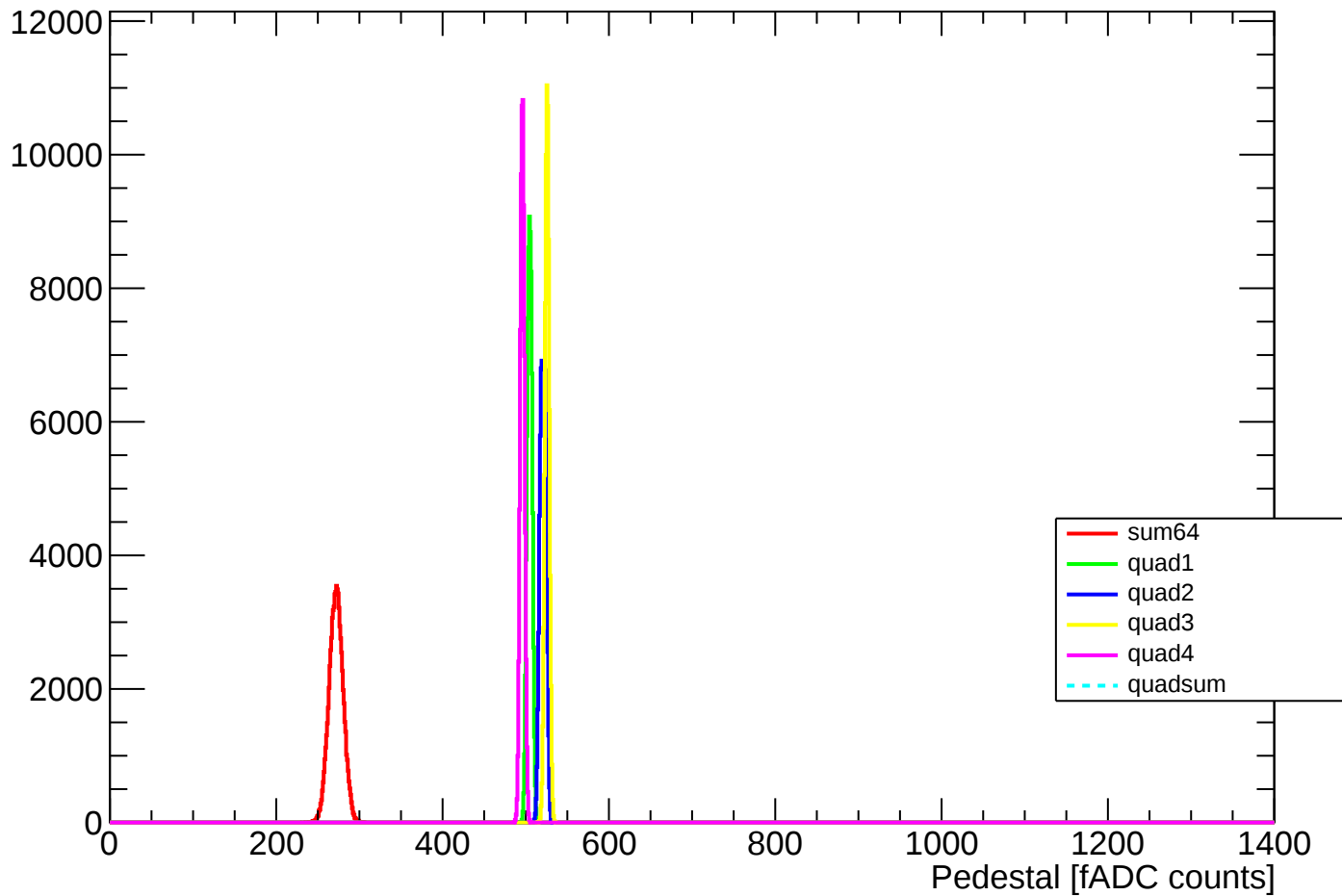
Pedestal Distribution (average fADC count between 0 - 24 ns)
