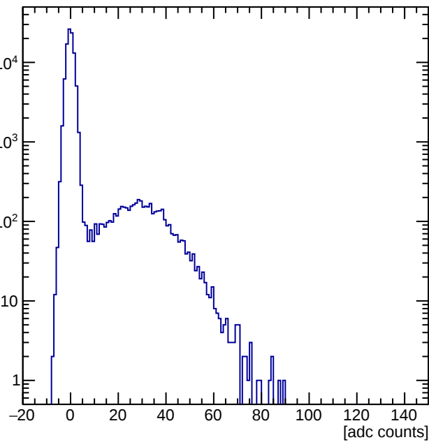
Pixel 51 ADC Spectrum (pedestal subtracted)
