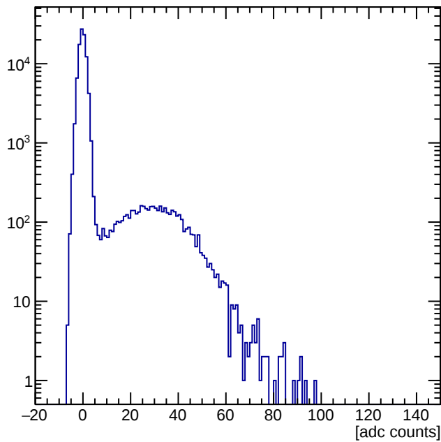
Pixel 49 ADC Spectrum (pedestal subtracted)
