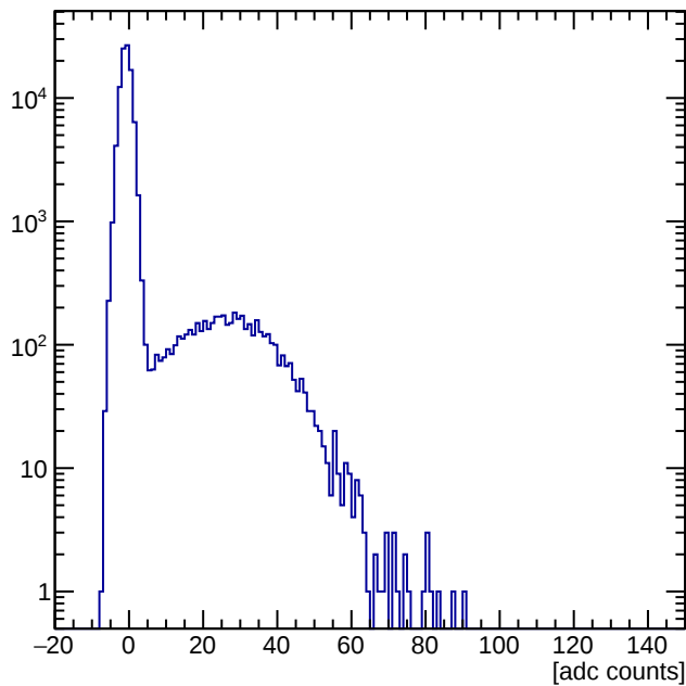
Pixel 50 ADC Spectrum (pedestal subtracted)
