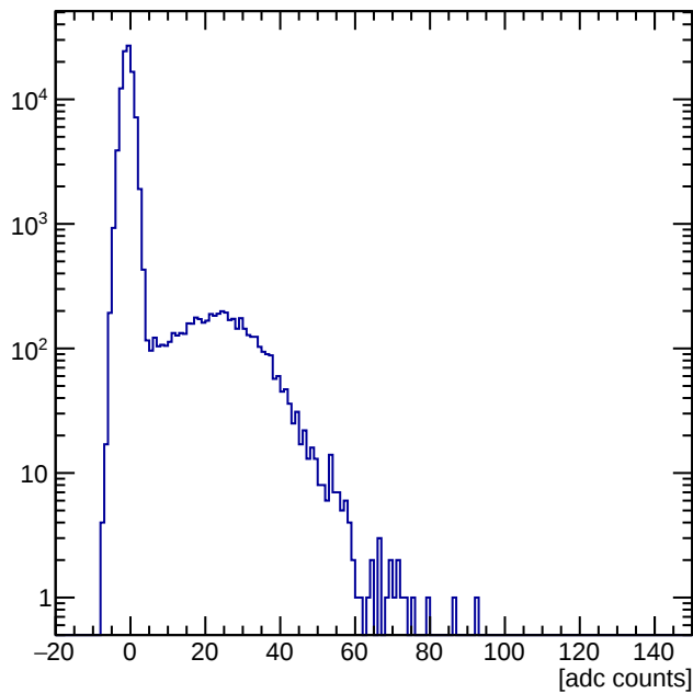
Pixel 52 ADC Spectrum (pedestal subtracted)
