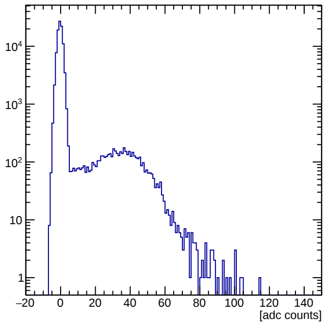
Pixel 60 ADC Spectrum (pedestal subtracted)
