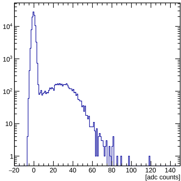
Pixel 58 ADC Spectrum (pedestal subtracted)
