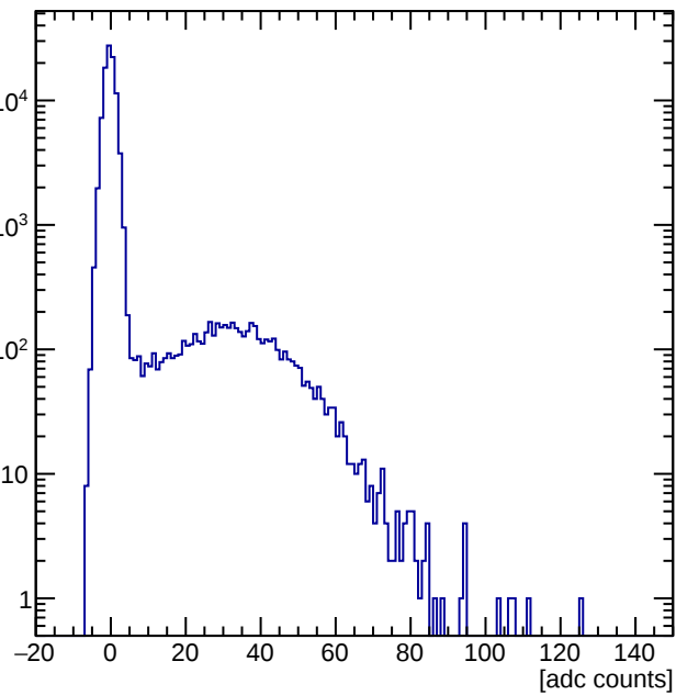
Pixel 59 ADC Spectrum (pedestal subtracted)
