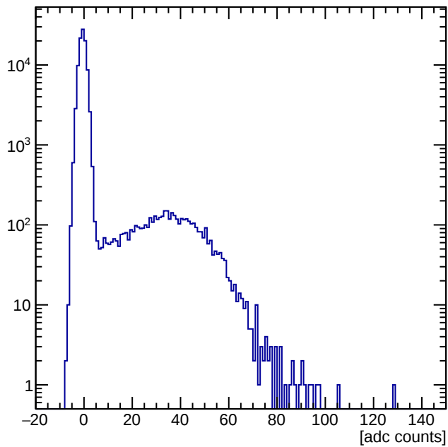
Pixel 57 ADC Spectrum (pedestal subtracted)
