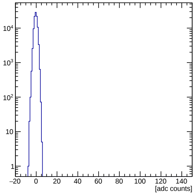
Pixel 51 ADC Spectrum (pedestal subtracted)
