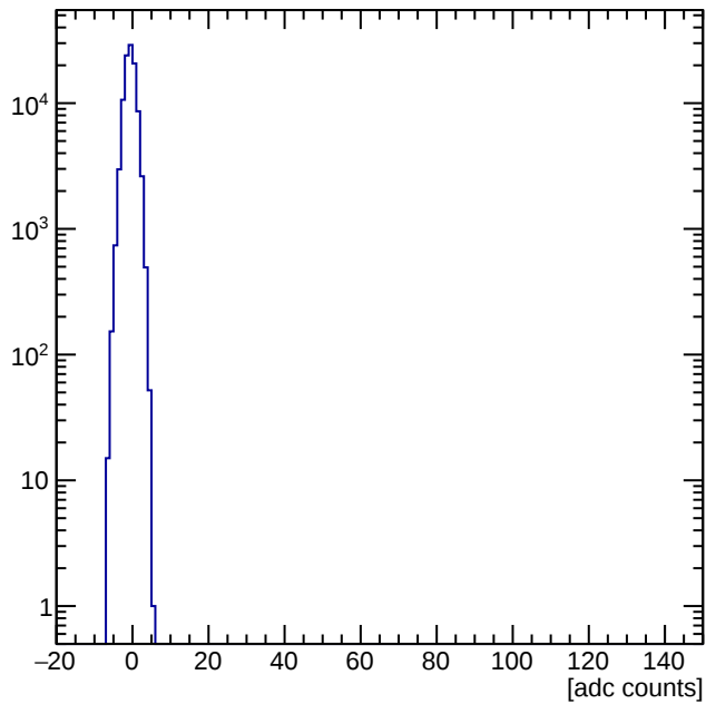
Pixel 59 ADC Spectrum (pedestal subtracted)
