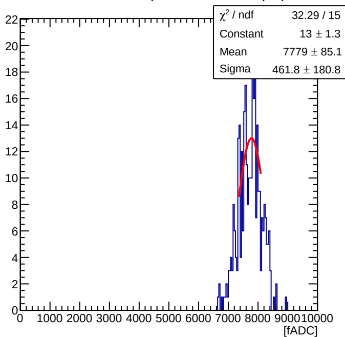
Maroc Sum of 56 ( Offline Sum = 2.74 pC )
