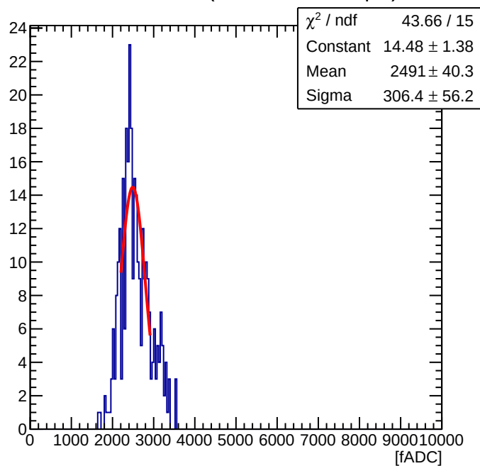
Maroc Sum of 56 ( Offline Sum = 0.56 pC )
