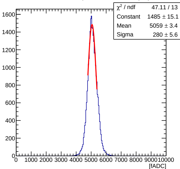
Maroc Sum of 56 ( Offline Sum = 1.59 pC )
