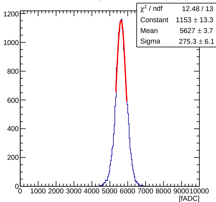
Maroc Sum of 56 ( Offline Sum = 1.81 pC )
