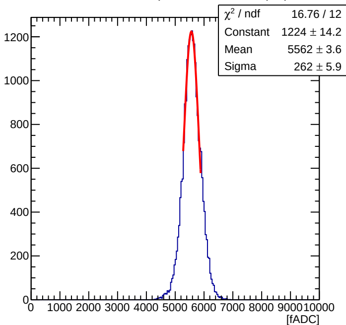
Maroc Sum of 56 ( Offline Sum = 1.79 pC )
