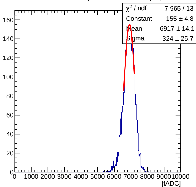
Maroc Sum of 56 ( Offline Sum = 2.34 pC )
