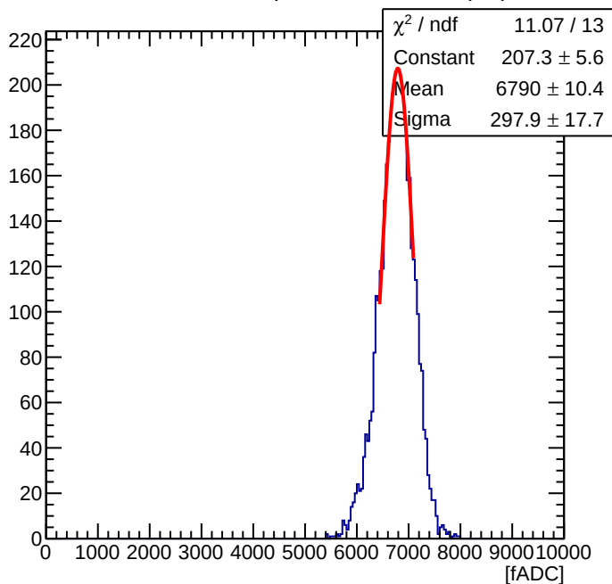
Maroc Sum of 56 ( Offline Sum = 2.29 pC )
