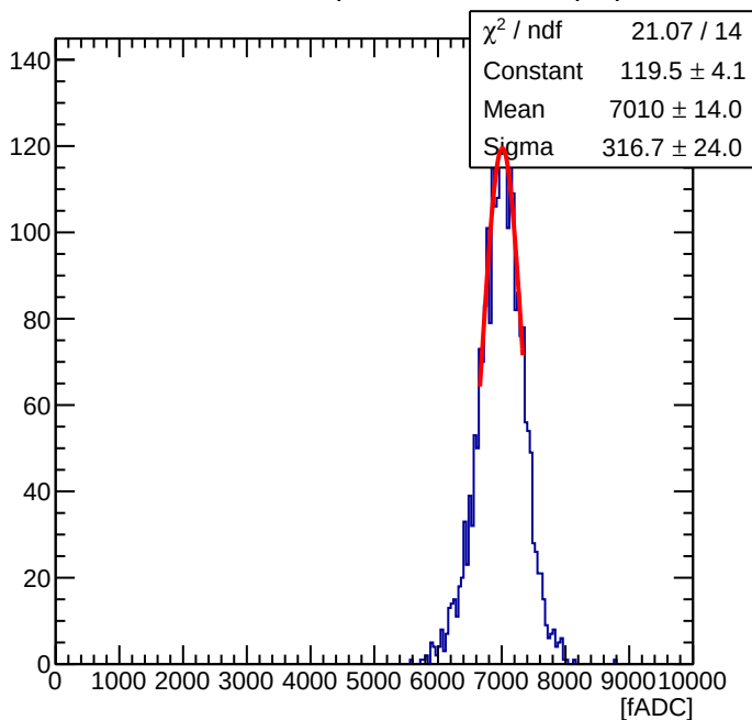
Maroc Sum of 56 ( Offline Sum = 2.39 pC )
