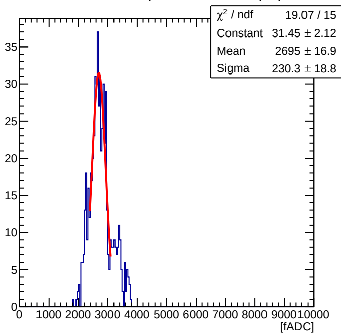
Maroc Sum of 56 ( Offline Sum = 0.64 pC )
