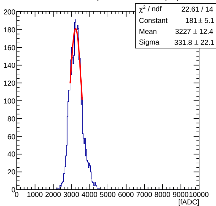
Maroc Sum of 56 ( Offline Sum = 0.86 pC )
