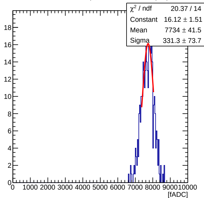
Maroc Sum of 56 ( Offline Sum = 2.71 pC )
