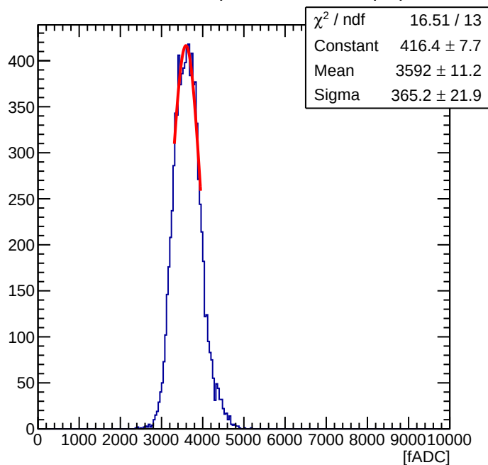
Maroc Sum of 56 ( Offline Sum = 1.01 pC )
