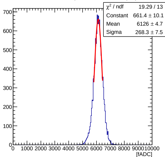
Maroc Sum of 56 ( Offline Sum = 2.01 pC )
