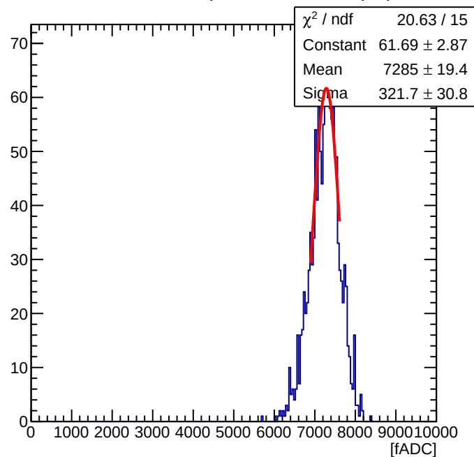
Maroc Sum of 56 ( Offline Sum = 2.51 pC )
