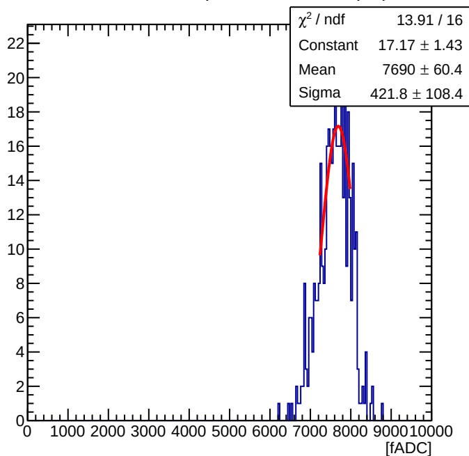
Maroc Sum of 56 ( Offline Sum = 2.69 pC )
