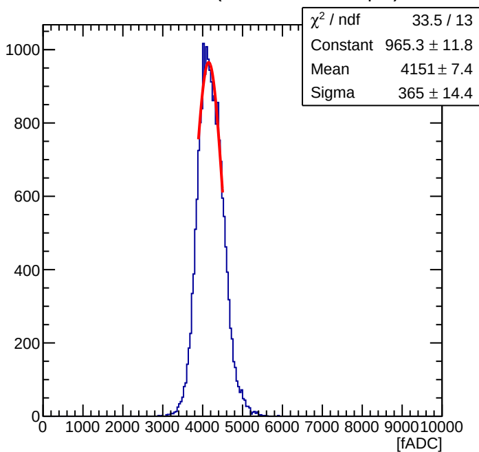
Maroc Sum of 56 ( Offline Sum = 1.24 pC )
