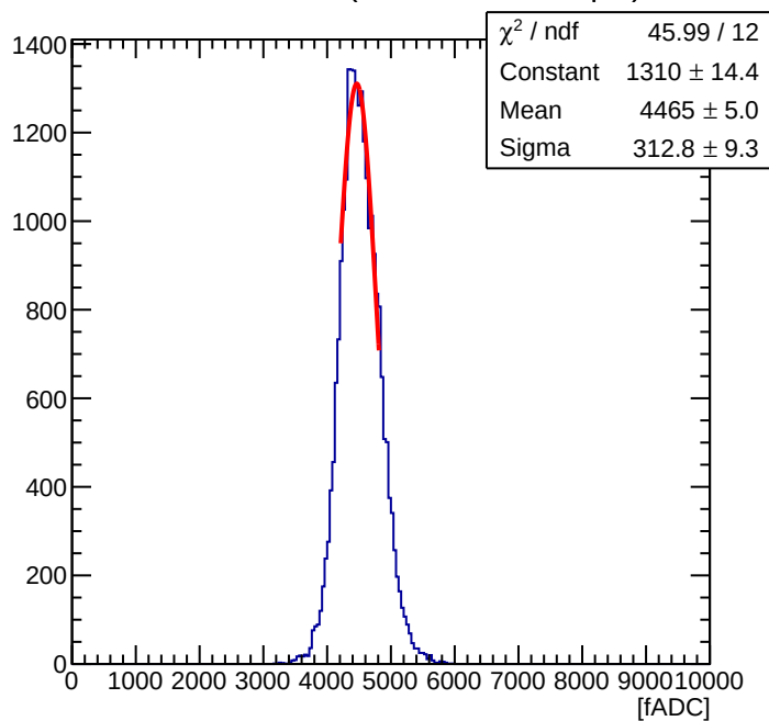
Maroc Sum of 56 ( Offline Sum = 1.36 pC )
