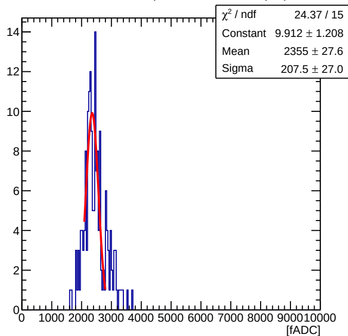
Maroc Sum of 56 ( Offline Sum = 0.51 pC )
