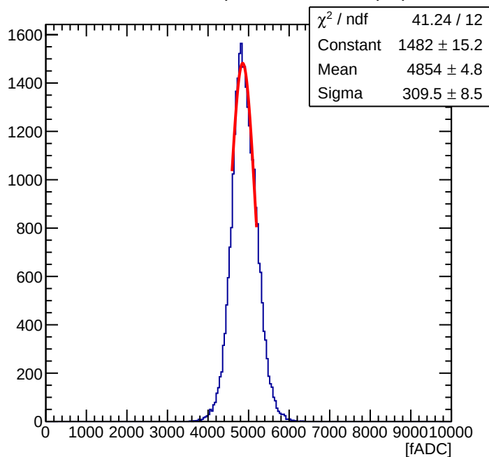
Maroc Sum of 56 ( Offline Sum = 1.51 pC )
