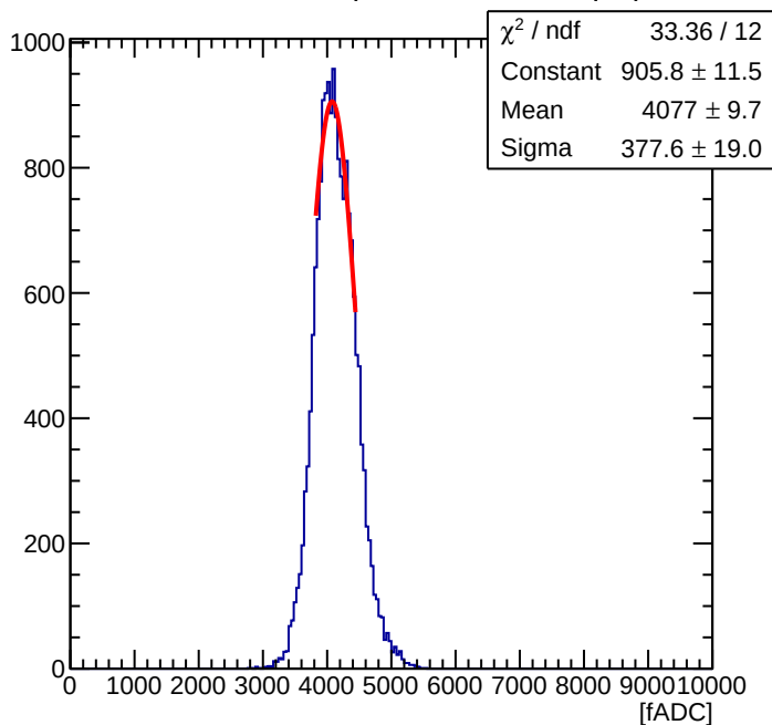
Maroc Sum of 56 ( Offline Sum = 1.21 pC )
