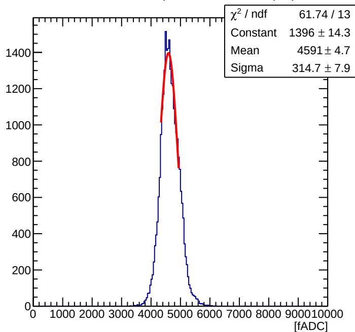
Maroc Sum of 56 ( Offline Sum = 1.41 pC )
