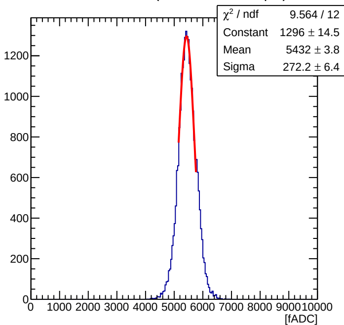
Maroc Sum of 56 ( Offline Sum = 1.74 pC )
