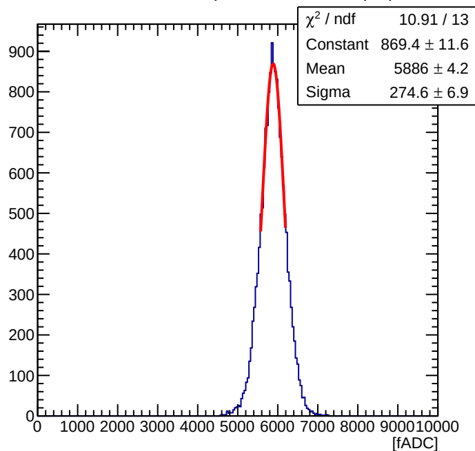
Maroc Sum of 56 ( Offline Sum = 1.91 pC )
