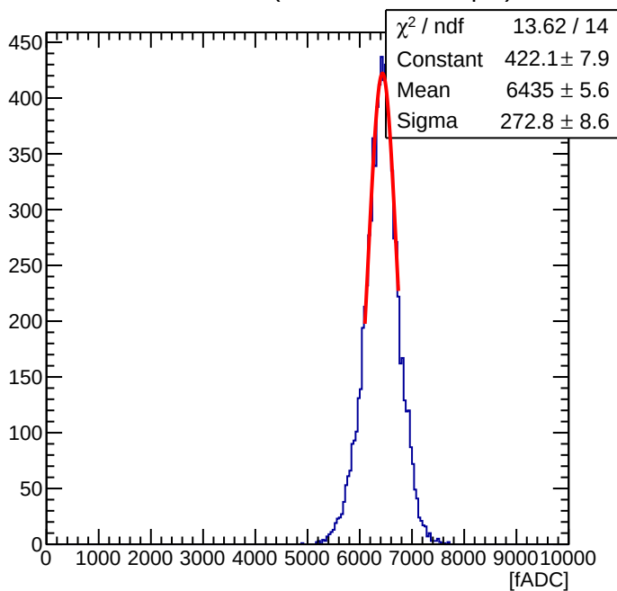
Maroc Sum of 56 ( Offline Sum = 2.14 pC )
