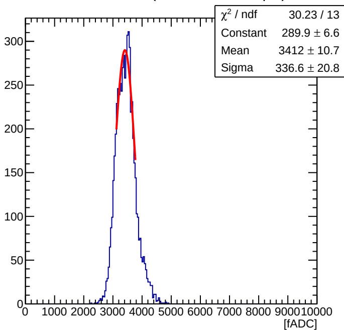
Maroc Sum of 56 ( Offline Sum = 0.94 pC )
