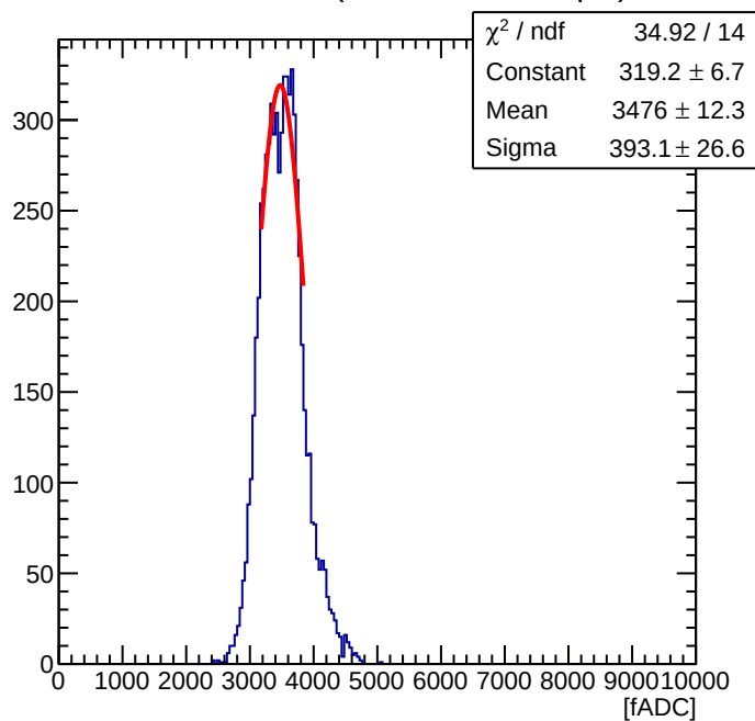
Maroc Sum of 56 ( Offline Sum = 0.96 pC )
