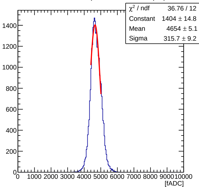
Maroc Sum of 56 ( Offline Sum = 1.44 pC )
