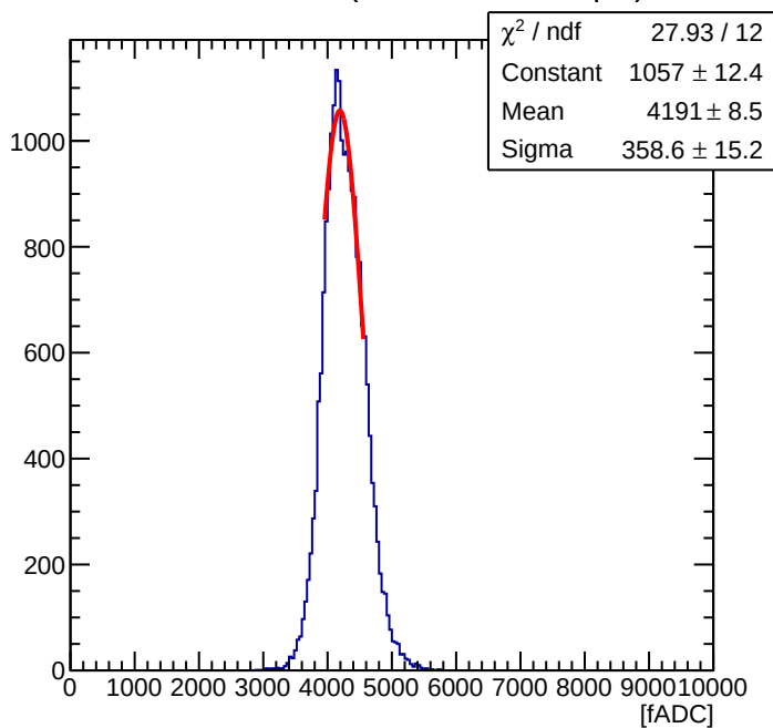
Maroc Sum of 56 ( Offline Sum = 1.26 pC )
