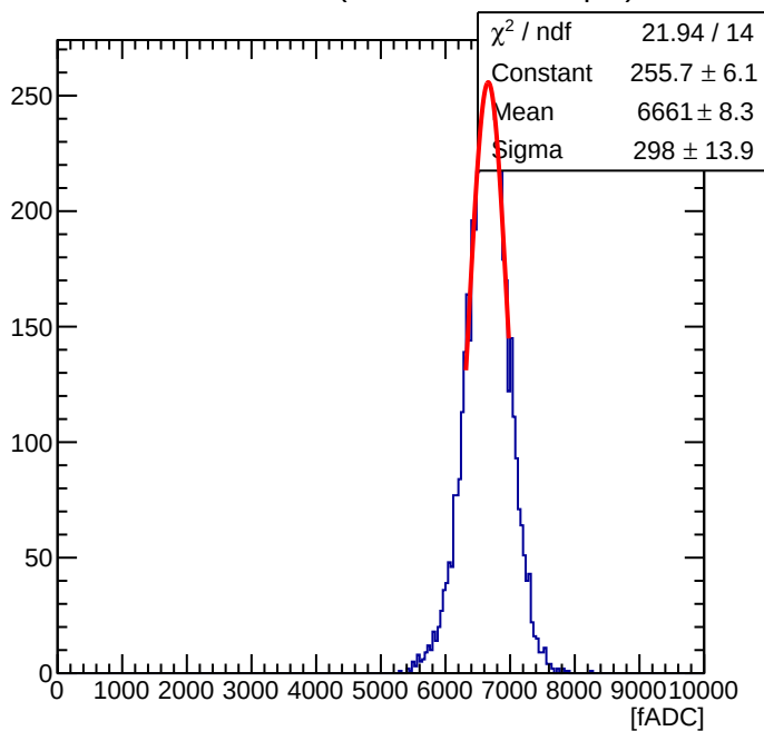
Maroc Sum of 56 ( Offline Sum = 2.24 pC )
