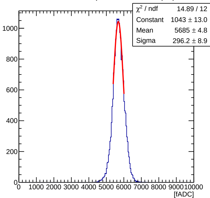
Maroc Sum of 56 ( Offline Sum = 1.84 pC )
