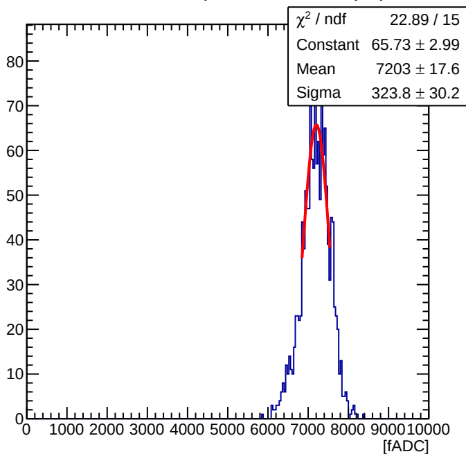
Maroc Sum of 56 ( Offline Sum = 2.49 pC )
