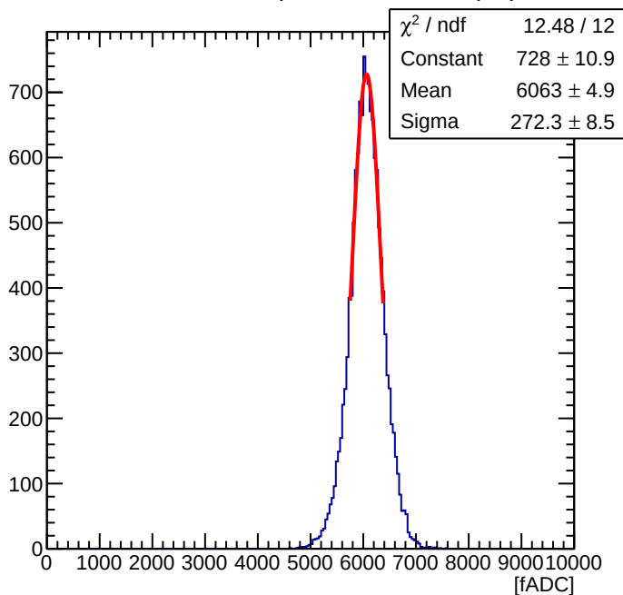
Maroc Sum of 56 ( Offline Sum = 1.99 pC )
