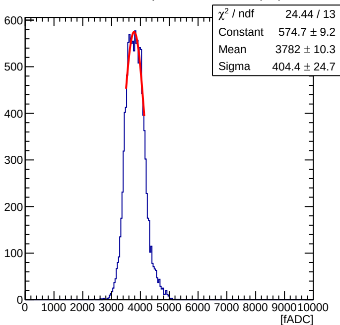
Maroc Sum of 56 ( Offline Sum = 1.09 pC )
