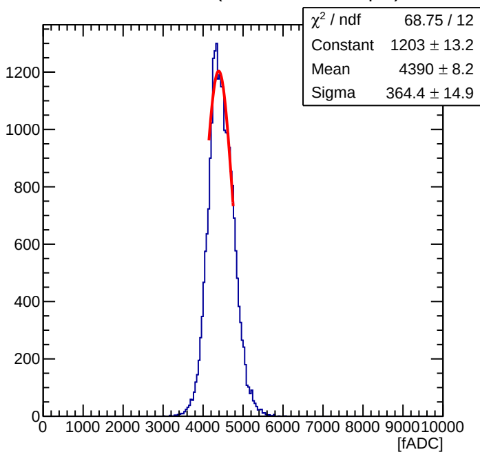
Maroc Sum of 56 ( Offline Sum = 1.34 pC )
