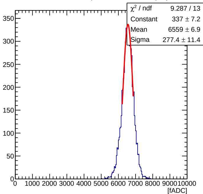
Maroc Sum of 56 ( Offline Sum = 2.19 pC )
