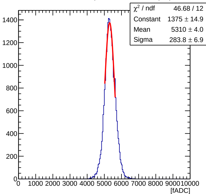
Maroc Sum of 56 ( Offline Sum = 1.69 pC )
