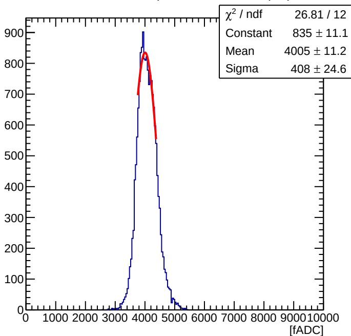
Maroc Sum of 56 ( Offline Sum = 1.19 pC )
