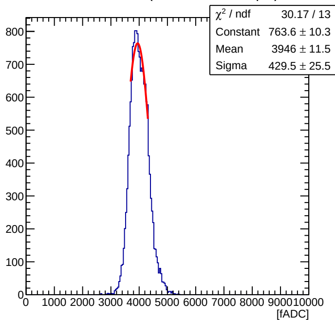
Maroc Sum of 56 ( Offline Sum = 1.16 pC )
