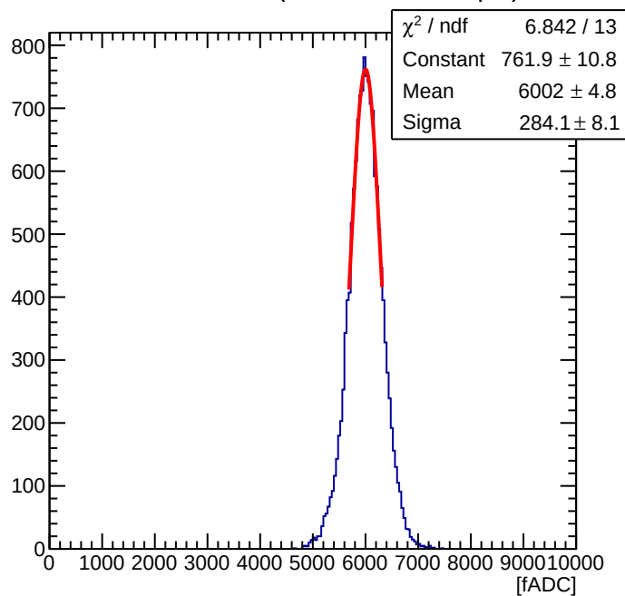
Maroc Sum of 56 ( Offline Sum = 1.96 pC )
