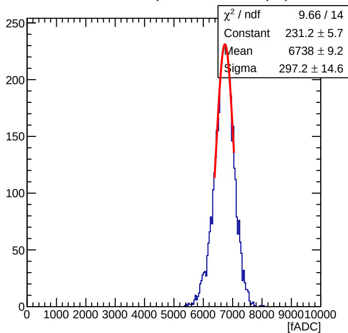
Maroc Sum of 56 ( Offline Sum = 2.26 pC )
