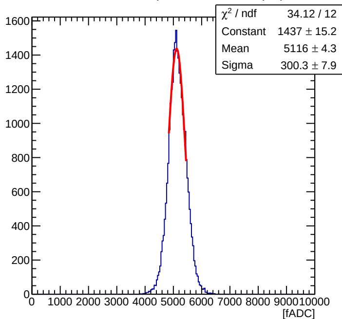
Maroc Sum of 56 ( Offline Sum = 1.61 pC )
