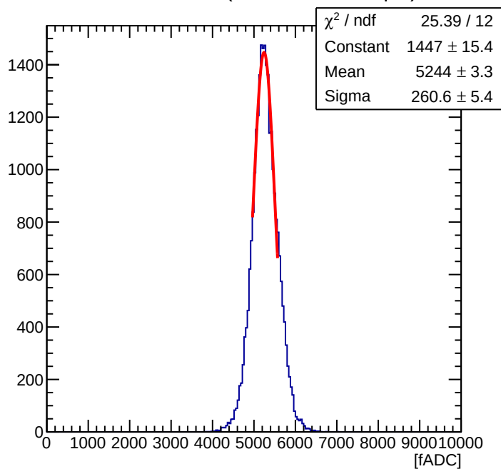
Maroc Sum of 56 ( Offline Sum = 1.66 pC )
