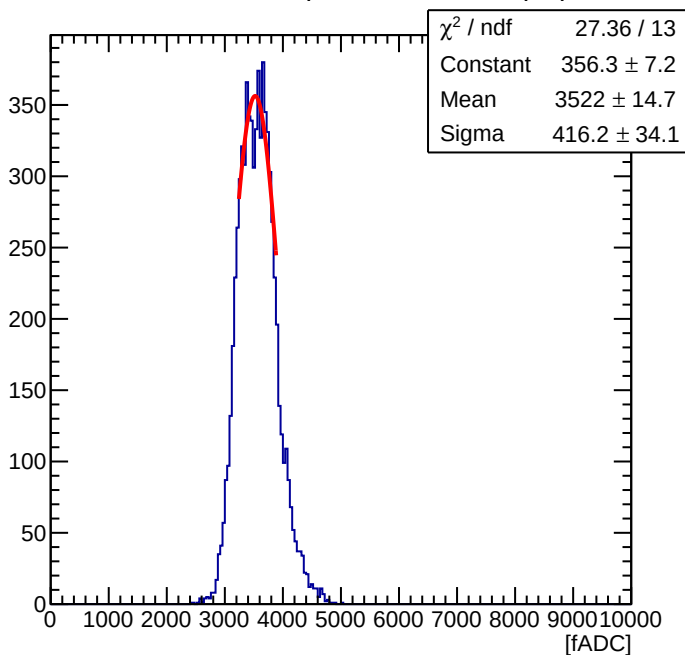
Maroc Sum of 56 ( Offline Sum = 0.99 pC )
