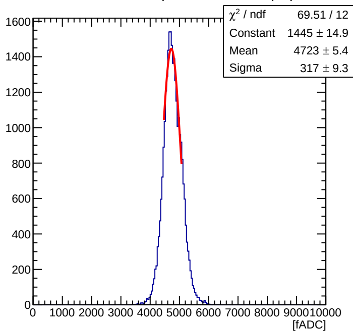
Maroc Sum of 56 ( Offline Sum = 1.46 pC )
