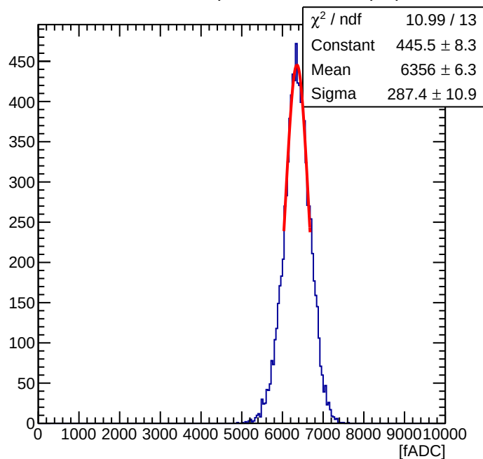
Maroc Sum of 56 ( Offline Sum = 2.11 pC )
