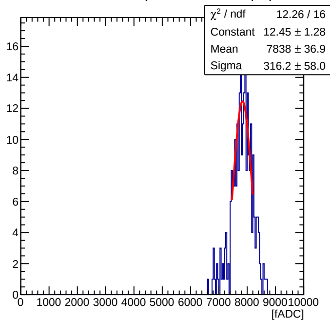
Maroc Sum of 56 ( Offline Sum = 2.76 pC )
