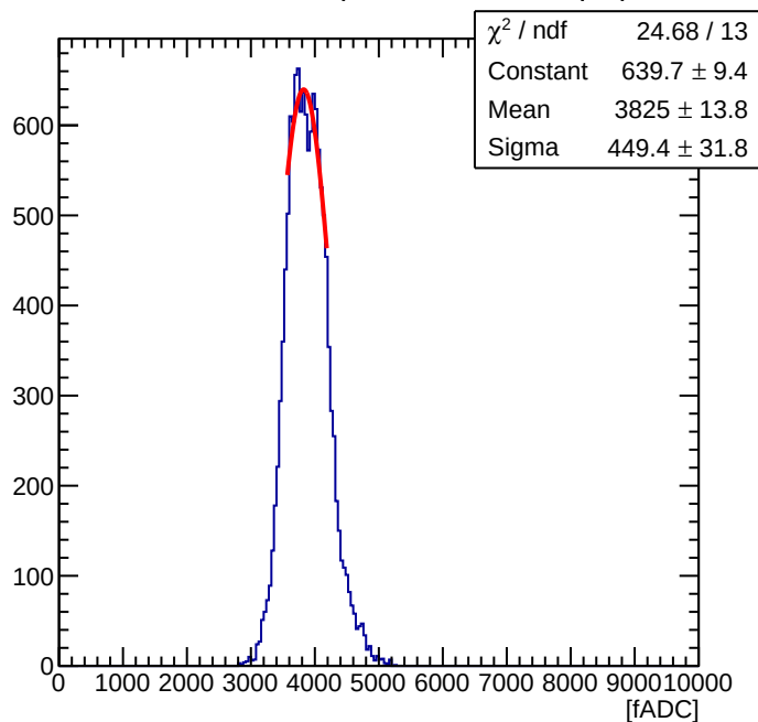
Maroc Sum of 56 ( Offline Sum = 1.11 pC )
