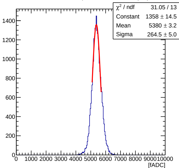
Maroc Sum of 56 ( Offline Sum = 1.71 pC )
