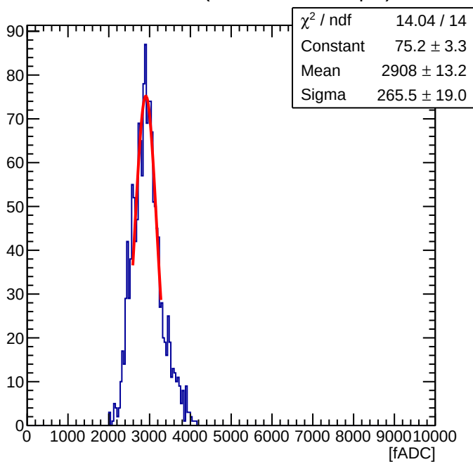
Maroc Sum of 56 ( Offline Sum = 0.74 pC )
