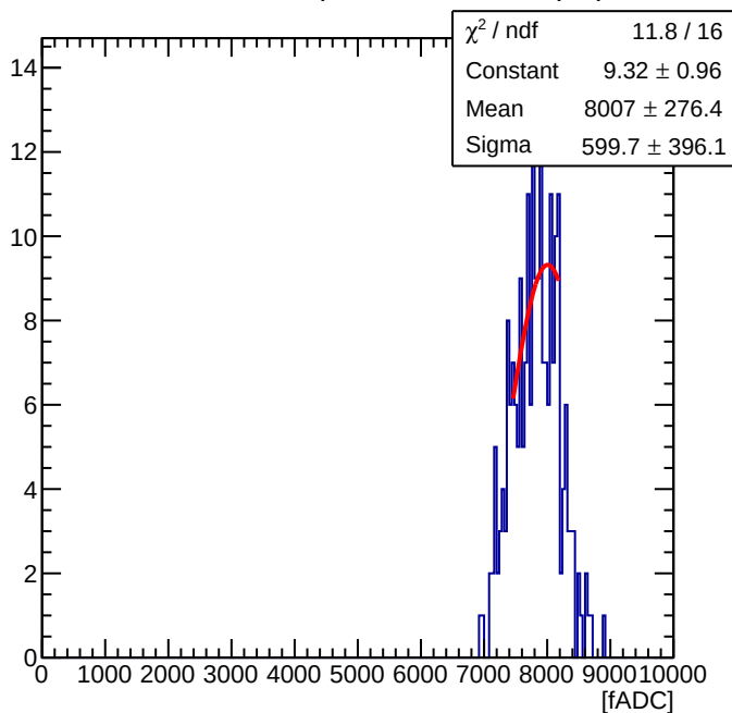
Maroc Sum of 56 ( Offline Sum = 2.79 pC )
