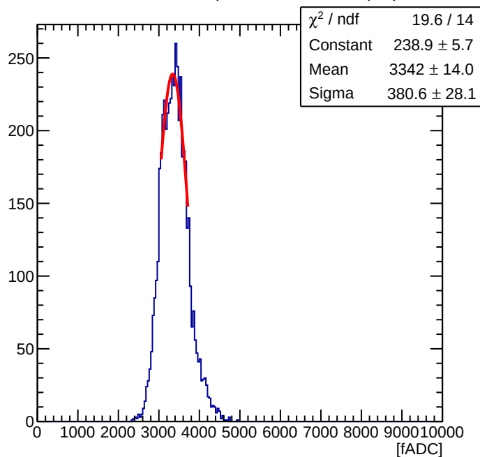
Maroc Sum of 56 ( Offline Sum = 0.91 pC )
