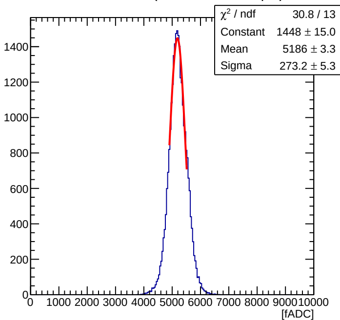
Maroc Sum of 56 ( Offline Sum = 1.64 pC )
