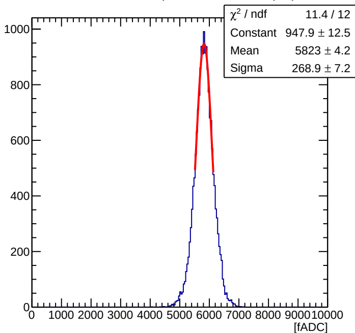
Maroc Sum of 56 ( Offline Sum = 1.89 pC )
