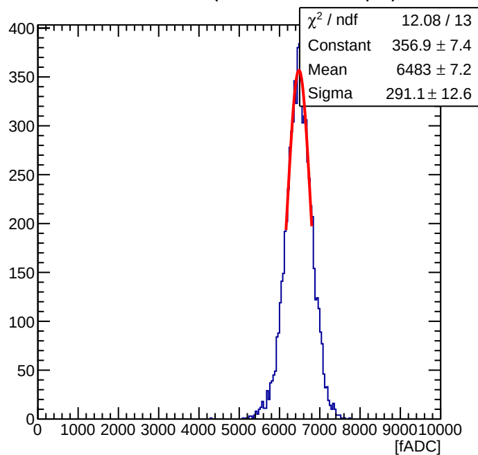
Maroc Sum of 56 ( Offline Sum = 2.16 pC )
