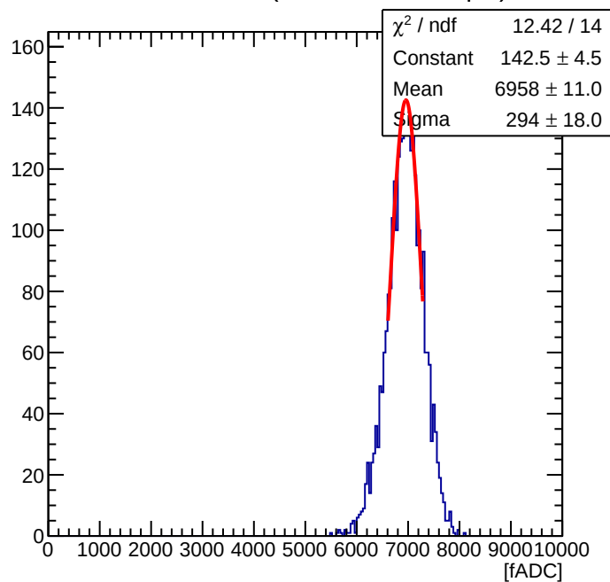
Maroc Sum of 56 ( Offline Sum = 2.36 pC )
