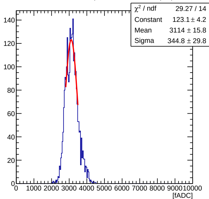
Maroc Sum of 56 ( Offline Sum = 0.81 pC )
