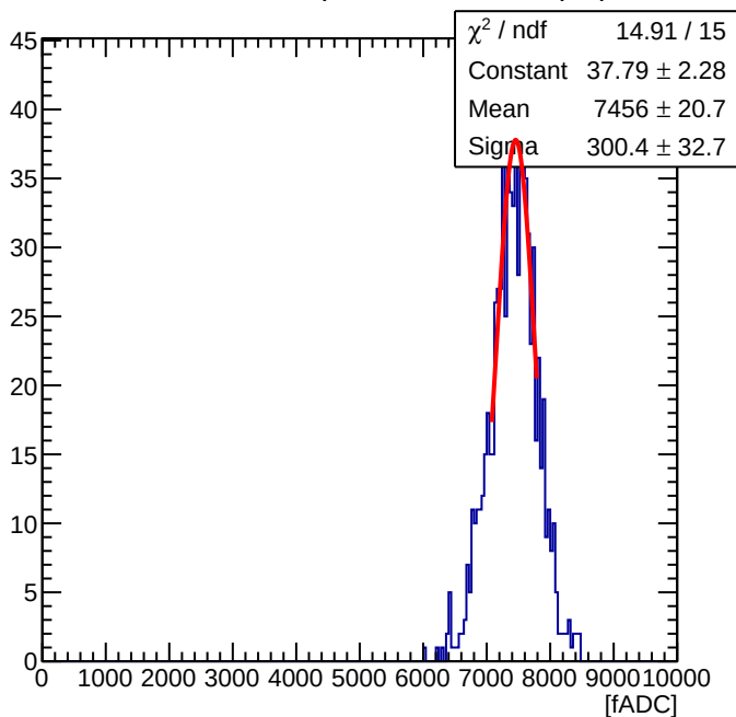
Maroc Sum of 56 ( Offline Sum = 2.59 pC )
