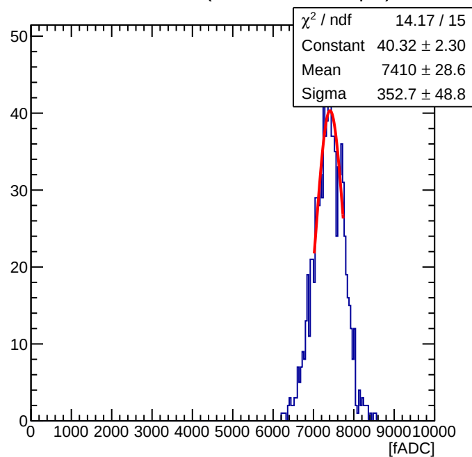
Maroc Sum of 56 ( Offline Sum = 2.56 pC )
