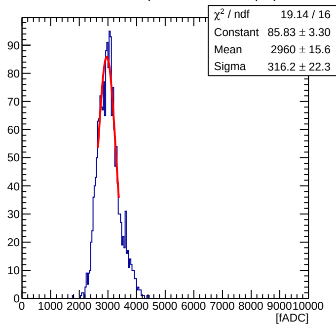
Maroc Sum of 56 ( Offline Sum = 0.76 pC )
