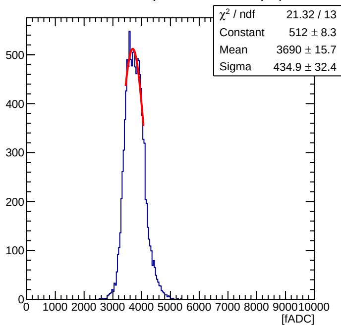
Maroc Sum of 56 ( Offline Sum = 1.06 pC )
