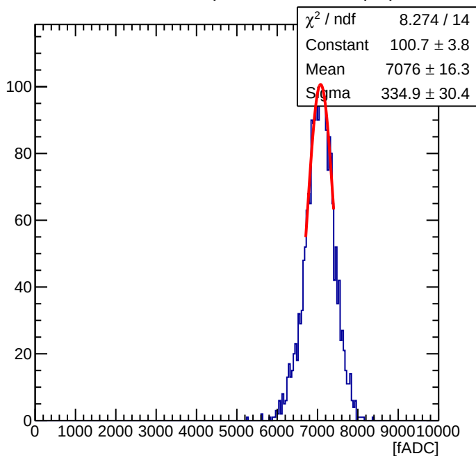
Maroc Sum of 56 ( Offline Sum = 2.41 pC )
