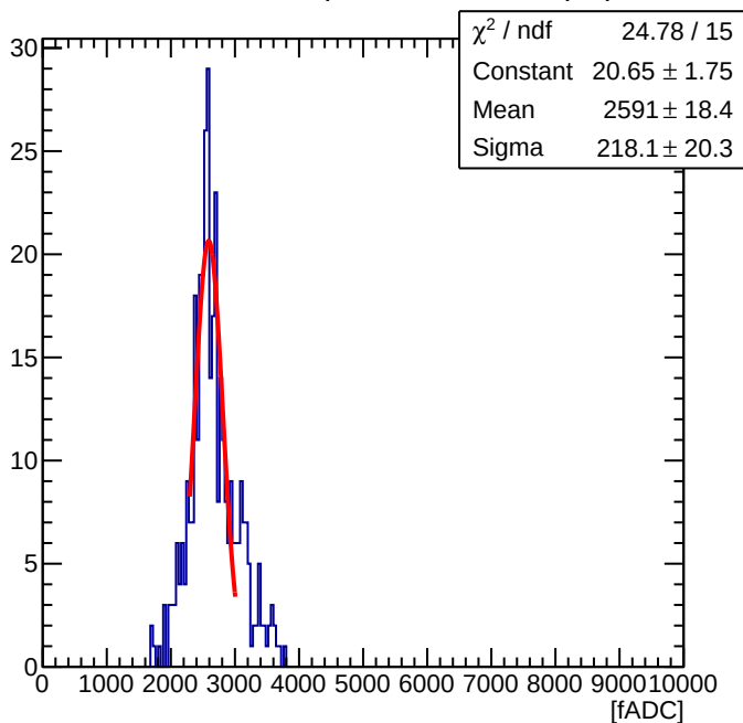
Maroc Sum of 56 ( Offline Sum = 0.59 pC )
