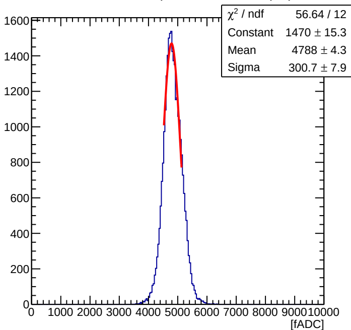
Maroc Sum of 56 ( Offline Sum = 1.49 pC )
