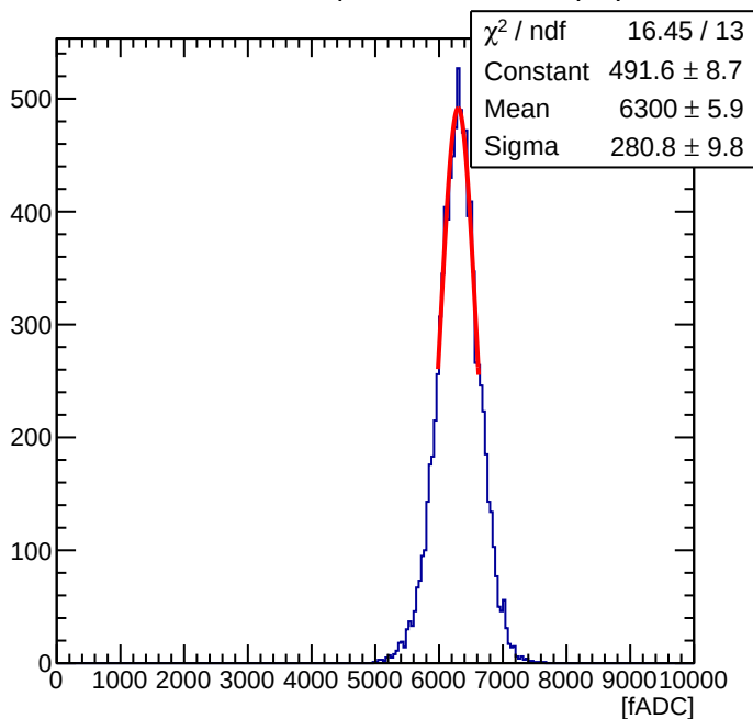
Maroc Sum of 56 ( Offline Sum = 2.09 pC )
