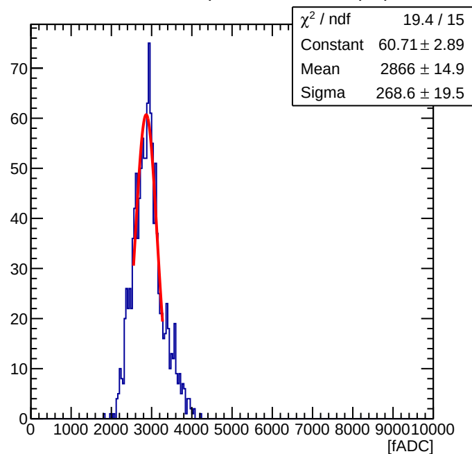
Maroc Sum of 56 ( Offline Sum = 0.71 pC )
