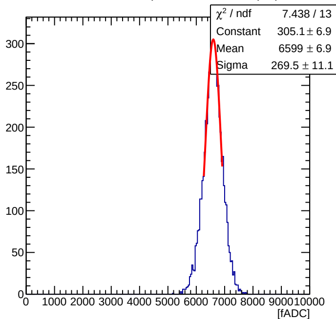
Maroc Sum of 56 ( Offline Sum = 2.21 pC )
