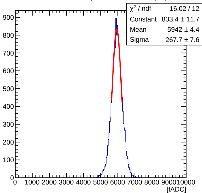
Maroc Sum of 56 ( Offline Sum = 1.94 pC )
