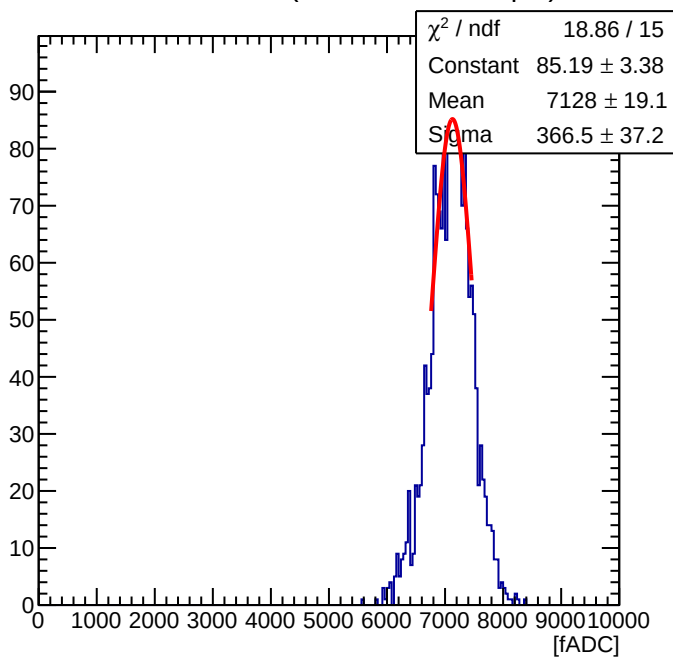
Maroc Sum of 56 ( Offline Sum = 2.44 pC )
