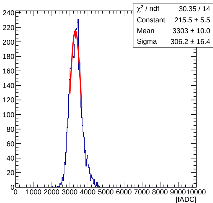
Maroc Sum of 56 ( Offline Sum = 0.89 pC )
