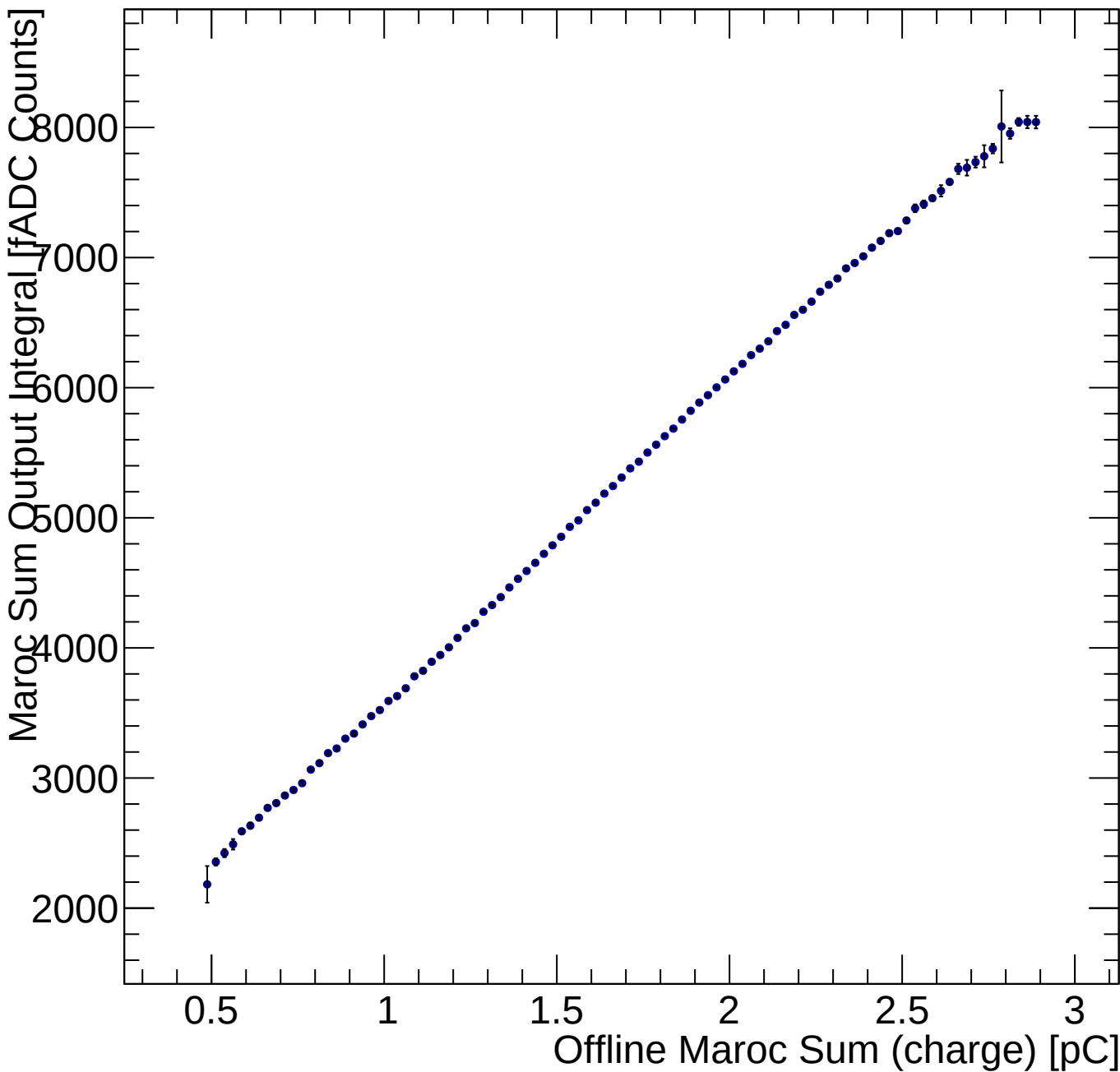
Maroc Sum of 56 fADC Counts vs. Charge
