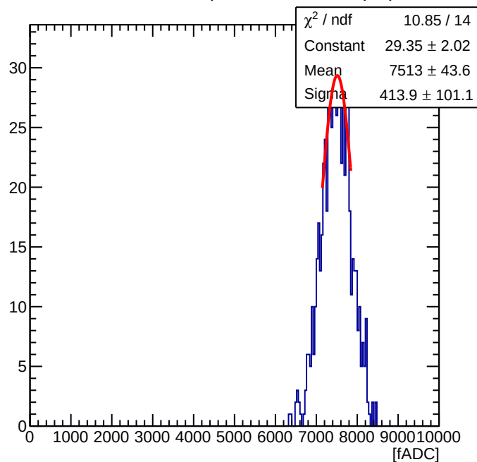
Maroc Sum of 56 ( Offline Sum = 2.61 pC )
