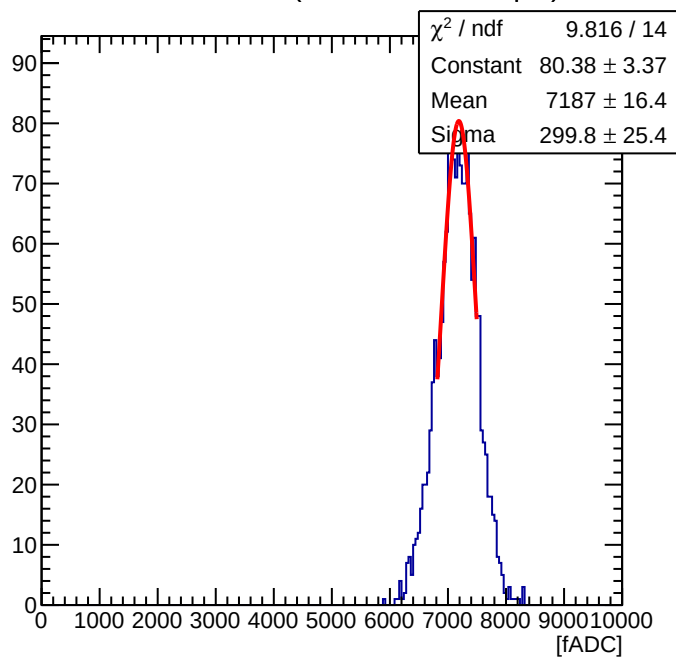
Maroc Sum of 56 ( Offline Sum = 2.46 pC )
