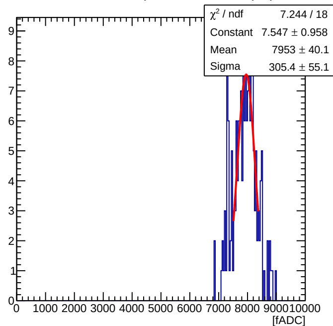
Maroc Sum of 56 ( Offline Sum = 2.81 pC )
