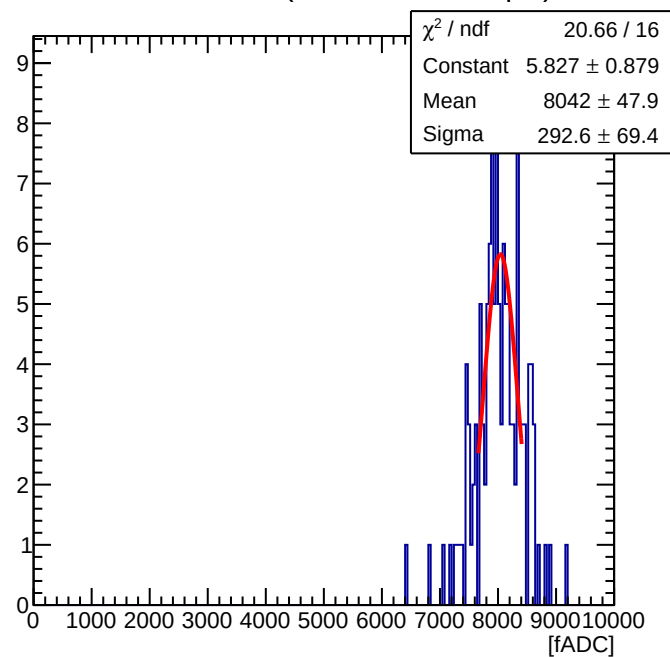
Maroc Sum of 56 ( Offline Sum = 2.86 pC )
