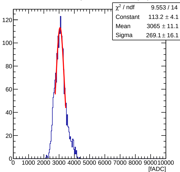
Maroc Sum of 56 ( Offline Sum = 0.79 pC )
