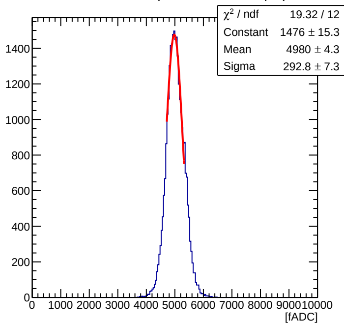
Maroc Sum of 56 ( Offline Sum = 1.56 pC )
