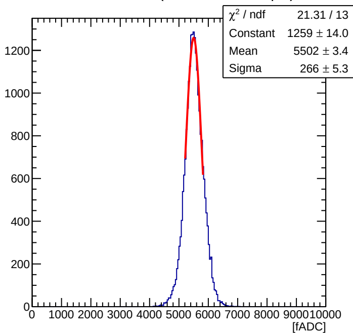
Maroc Sum of 56 ( Offline Sum = 1.76 pC )
