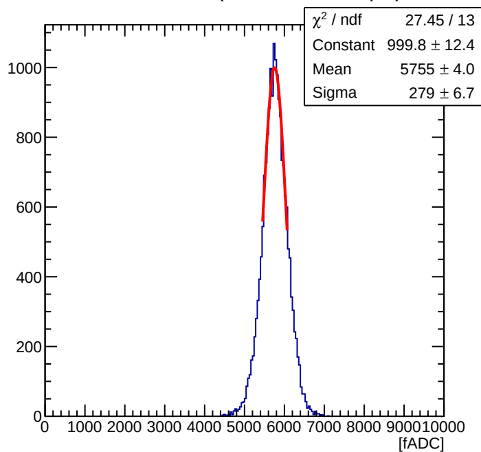
Maroc Sum of 56 ( Offline Sum = 1.86 pC )
