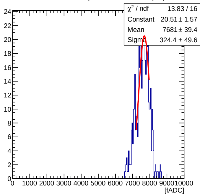
Maroc Sum of 56 ( Offline Sum = 2.66 pC )
