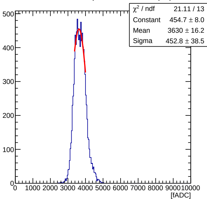
Maroc Sum of 56 ( Offline Sum = 1.04 pC )
