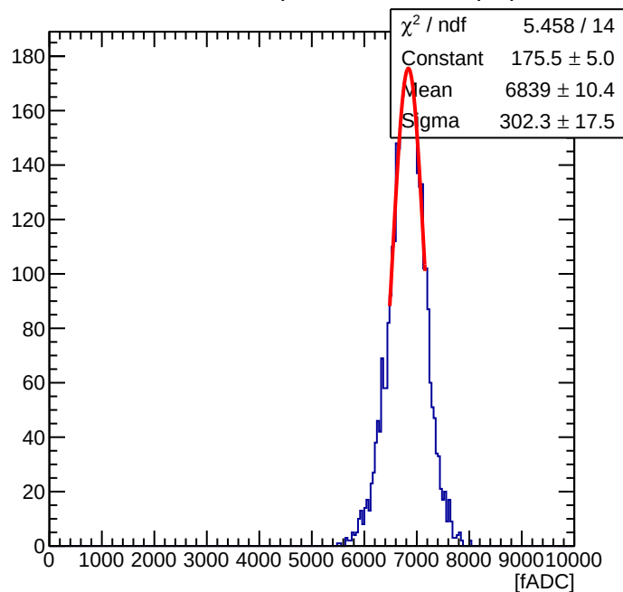
Maroc Sum of 56 ( Offline Sum = 2.31 pC )
