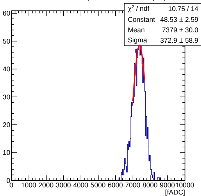
Maroc Sum of 56 ( Offline Sum = 2.54 pC )
