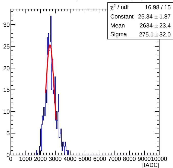
Maroc Sum of 56 ( Offline Sum = 0.61 pC )
