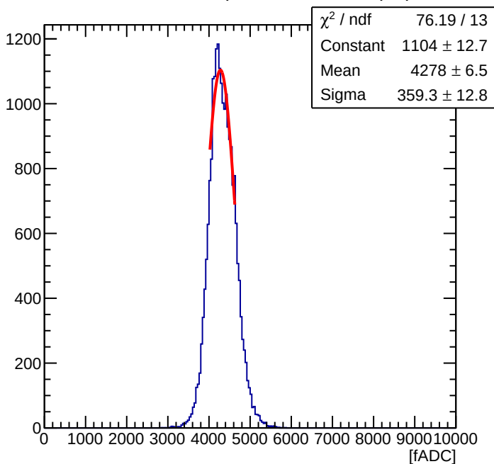
Maroc Sum of 56 ( Offline Sum = 1.29 pC )
