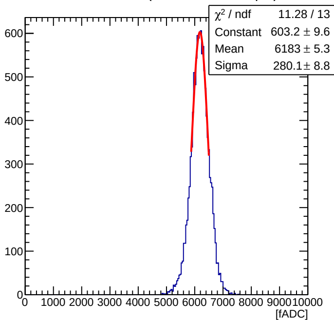
Maroc Sum of 56 ( Offline Sum = 2.04 pC )
