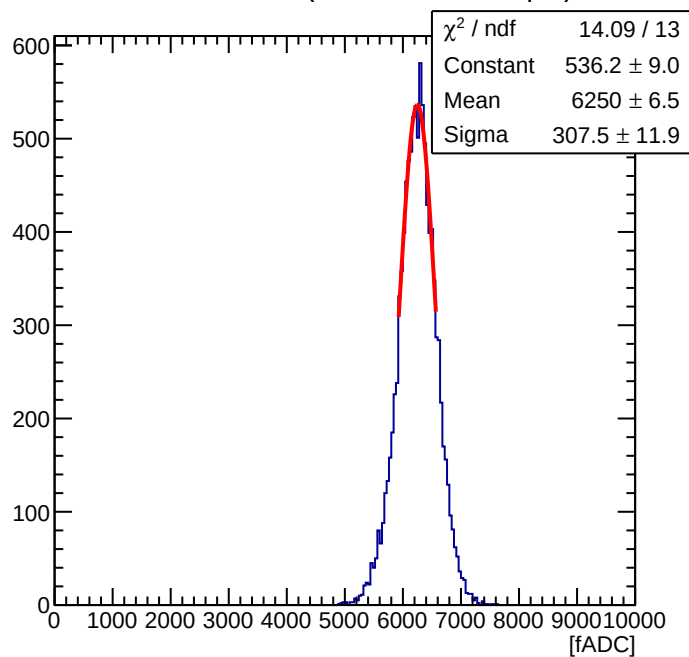
Maroc Sum of 56 ( Offline Sum = 2.06 pC )
