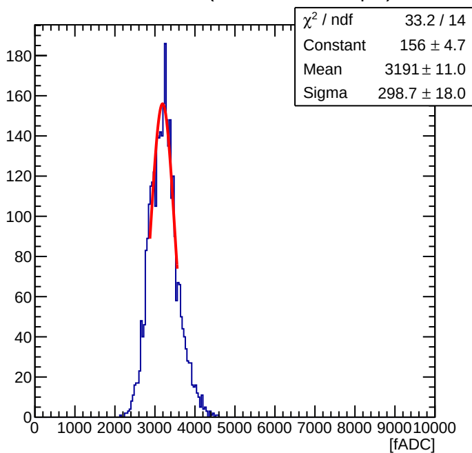
Maroc Sum of 56 ( Offline Sum = 0.84 pC )
