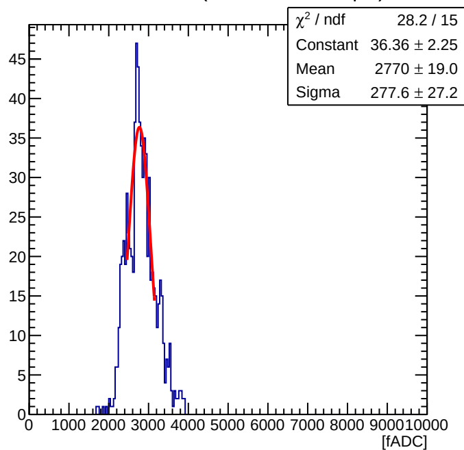
Maroc Sum of 56 ( Offline Sum = 0.66 pC )
