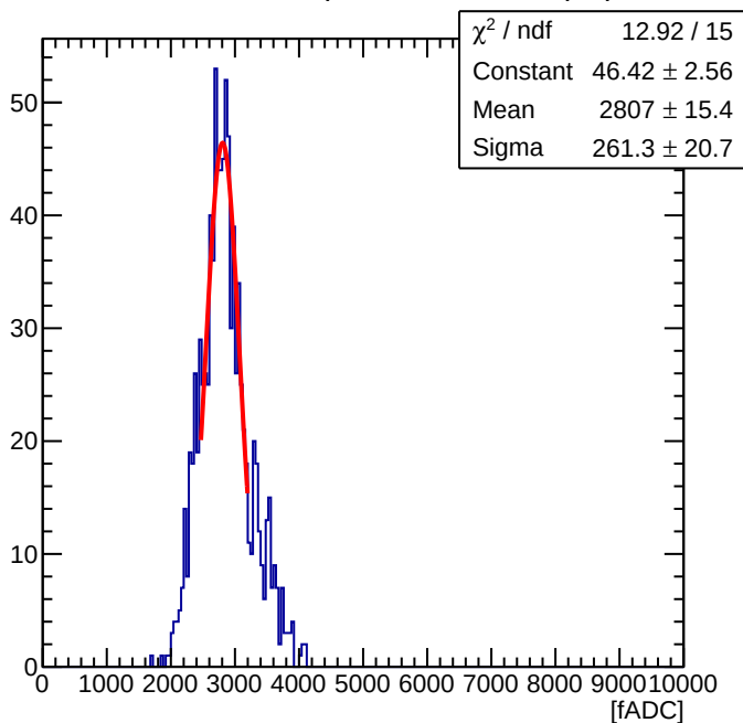
Maroc Sum of 56 ( Offline Sum = 0.69 pC )
