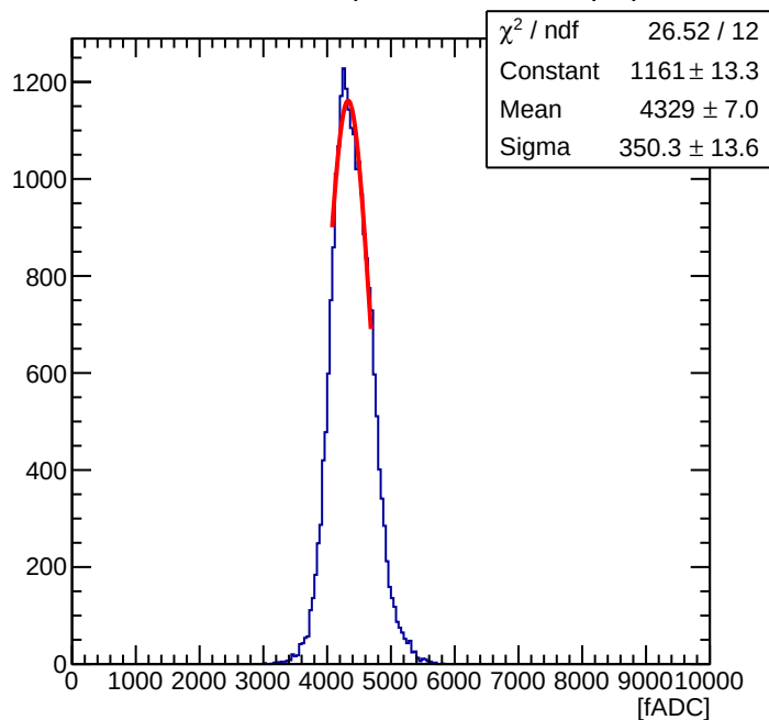
Maroc Sum of 56 ( Offline Sum = 1.31 pC )
