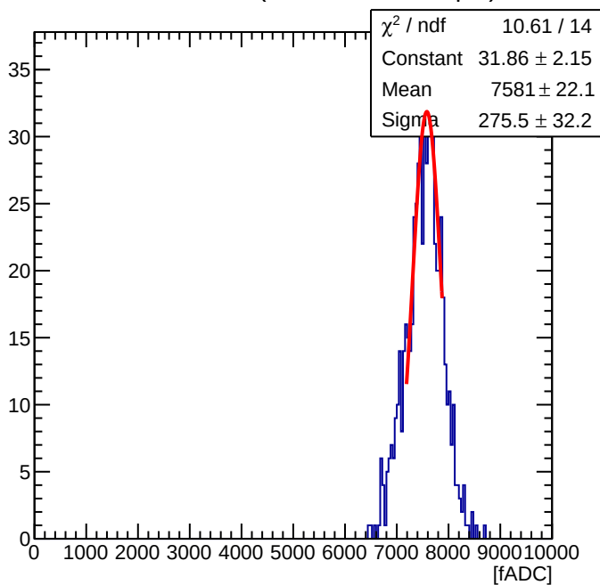
Maroc Sum of 56 ( Offline Sum = 2.64 pC )
