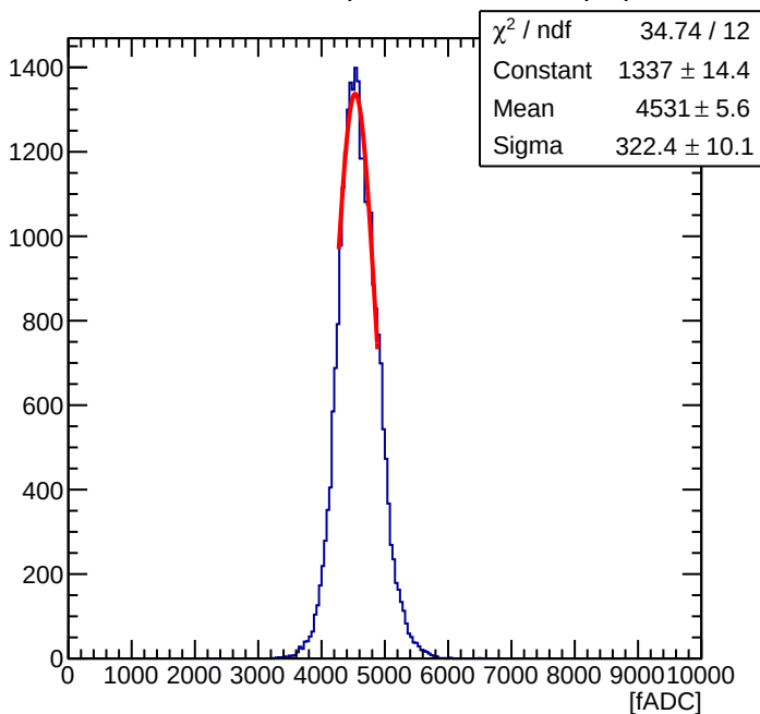
Maroc Sum of 56 ( Offline Sum = 1.39 pC )
