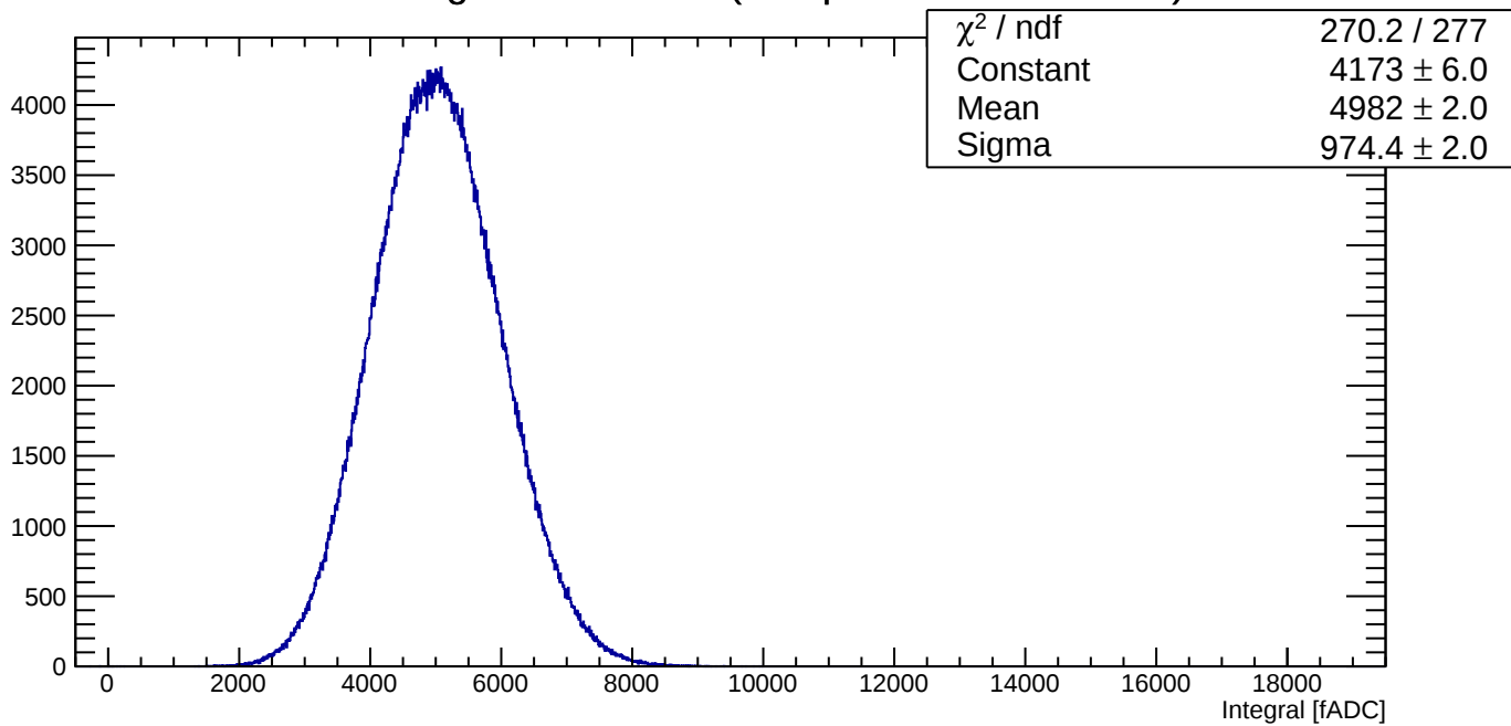
fADC Integral Distribution (with pedestal subtraction)
