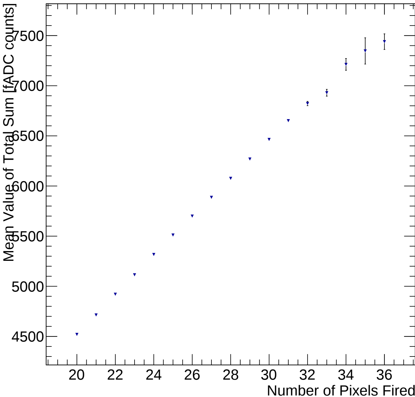
Maroc Sum of 56 fADC Counts vs. Number of Pixels Fired
