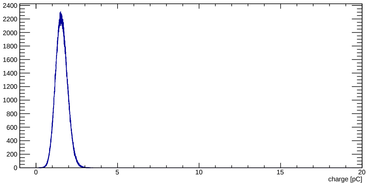
Sum of 56 Maroc Channels (adcPedSub)
