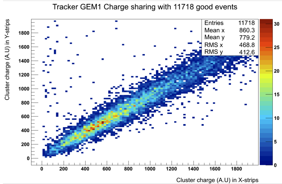
Figure 66: The charge division between x and y stripes for the 40×50 cm 2 GEM chamber.
