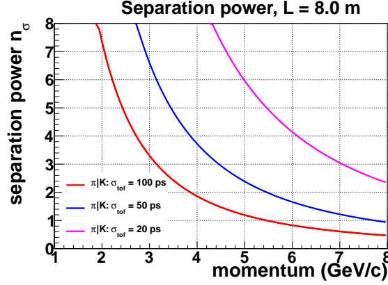
Figure 36: Kaon identification by TOF.
