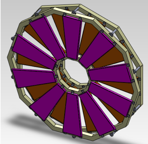
Figure 62: The GEM module arrangement at one of the detector locations of the SoLID SIDIS configuration
