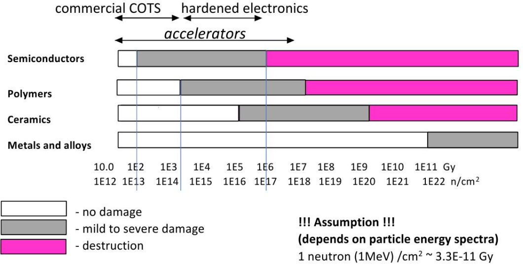
Figure 136: Estimate of the tolerance of different material to different level of radiation exposure given in Gy and \frac{\text{neutron}(1\text{MeV})}{\text{cm}^2} . This is just a first order approximation and a detailed analysis of each equipment is needed in order to establish the correct radiation tolerance of each detector/material
