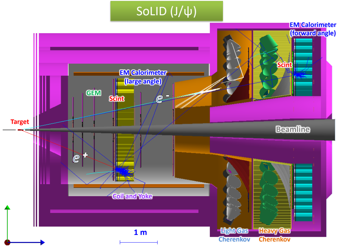
Figure 44: The experimental layout for the SoLID J/\psi setup based on the CLEO-II magnet. It is similar to that of the SIDIS- ^3\text{He} setup, except that the ^3\text{He} target is replaced by the standard Hall A 15 cm liquid Hydrogen target upstream in front of the spectrometer entrance.
