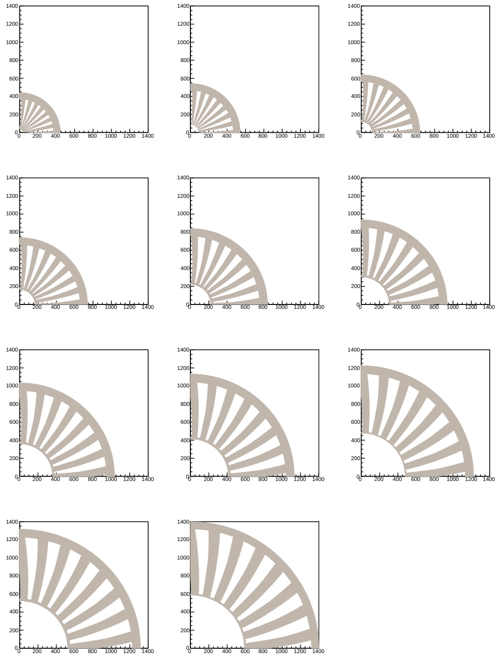
Figure 54: Face on views (first quadrant only) of the 11 plates in the PVDIS baffle system.
