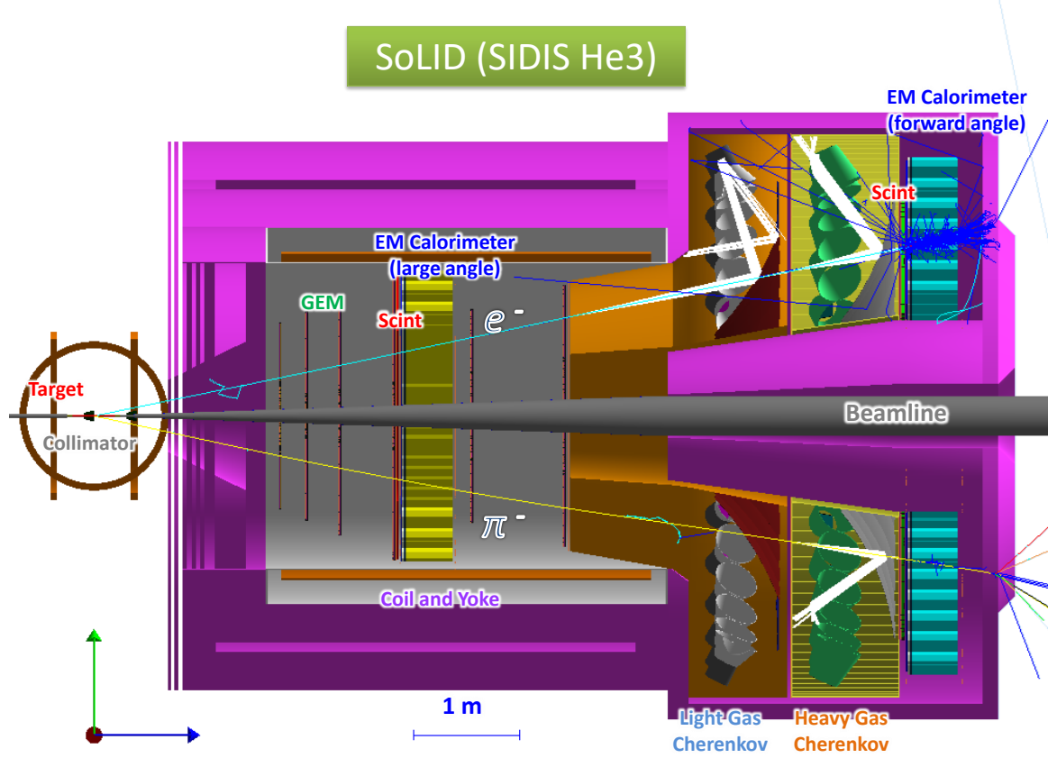
Figure 37: The experimental layout of the SoLID SIDIS- ^3\text{He} setup based on the CLEO magnet. The scattered electrons are detected by both forward-angle and large-angle detectors. The leading pions are detected by the forward-angle detector only. The polarized ^3\text{He} target will be placed upstream in front of the spectrometer entrance.
