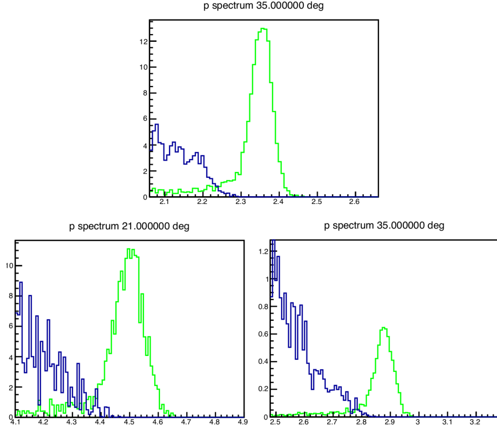
Figure 167: Elastic (green) and inelastic (blue) spectra for 4.4 GeV (top) and 6.6 GeV (bottom) electrons on a hydrogen target, at scattering angles of 21° (bottom left) and 35° (top and bottom right).
