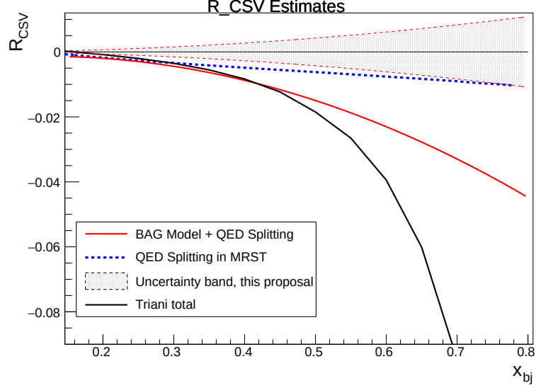
Figure 26: Possible contribution to A_{PV} due to CSV. The largest prediction comes from Ref. [116]
