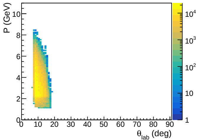
decay lepton -
