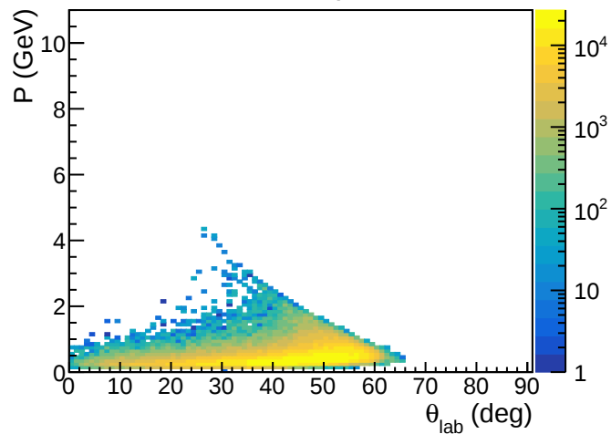
recoil p
