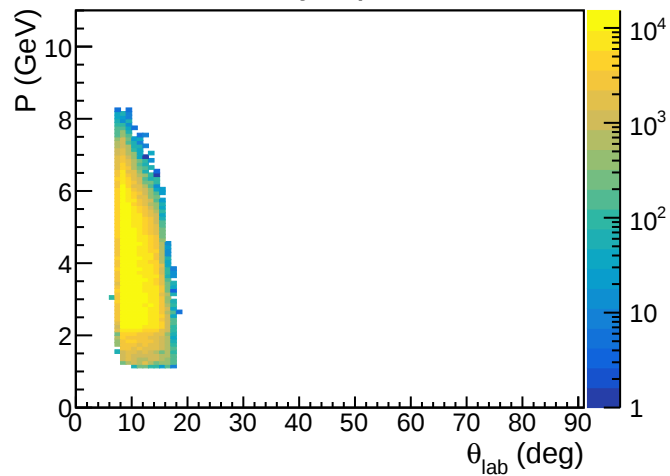
decay lepton +
