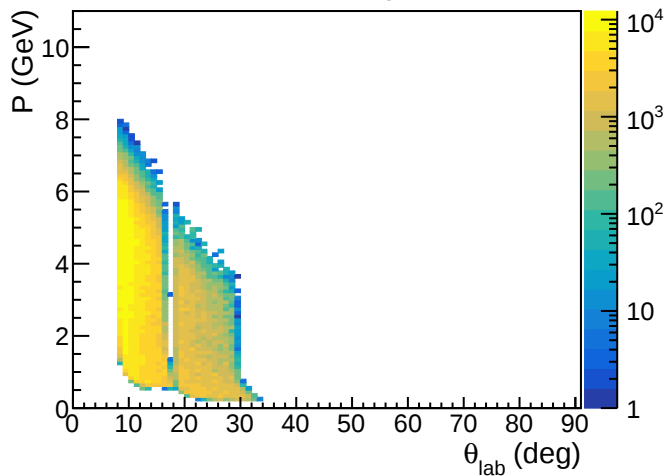
scattered lepton
