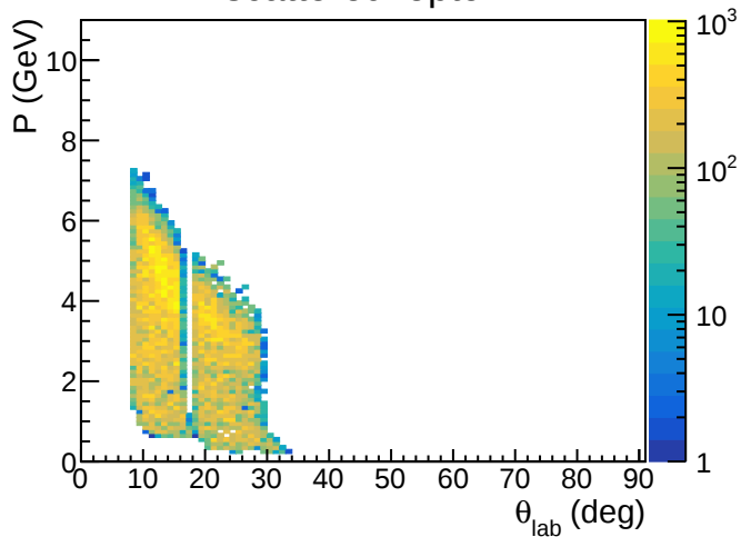
decay lepton -
