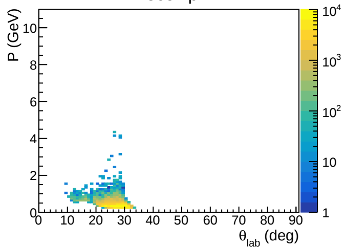
decay lepton +
