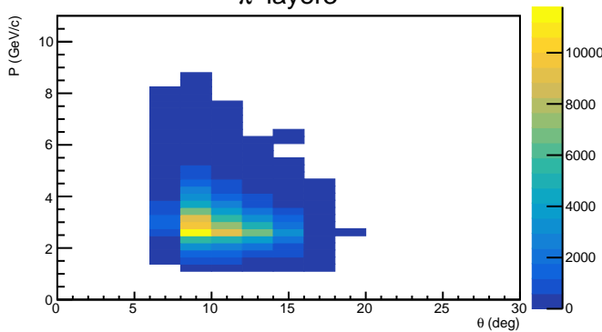
\pi^- layer3
