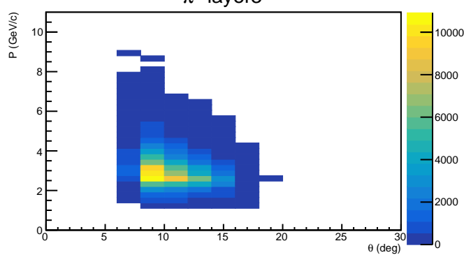
\pi^+ layer3
