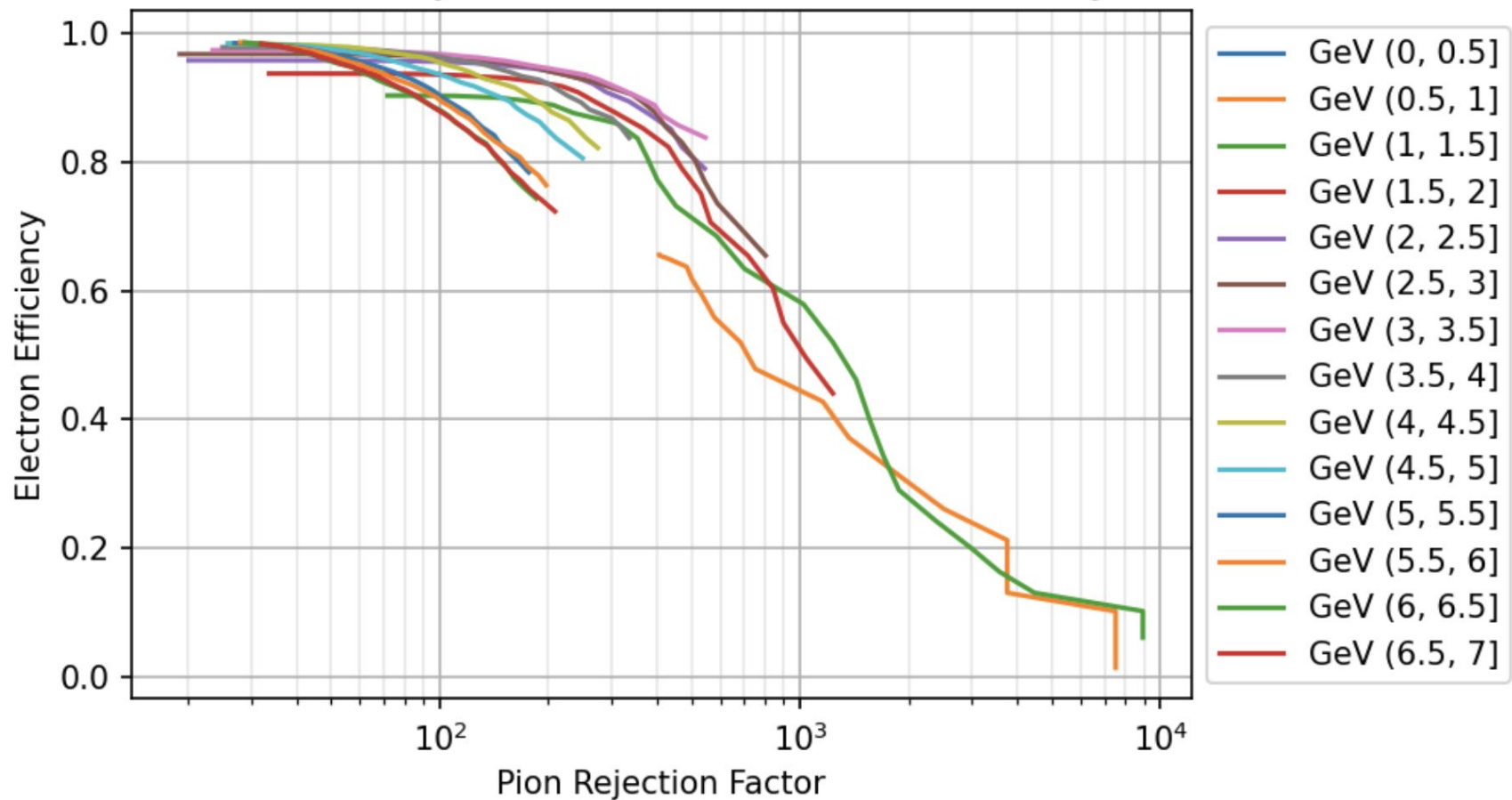
TS3 Pion Rejection Factor vs Electron Efficiency
